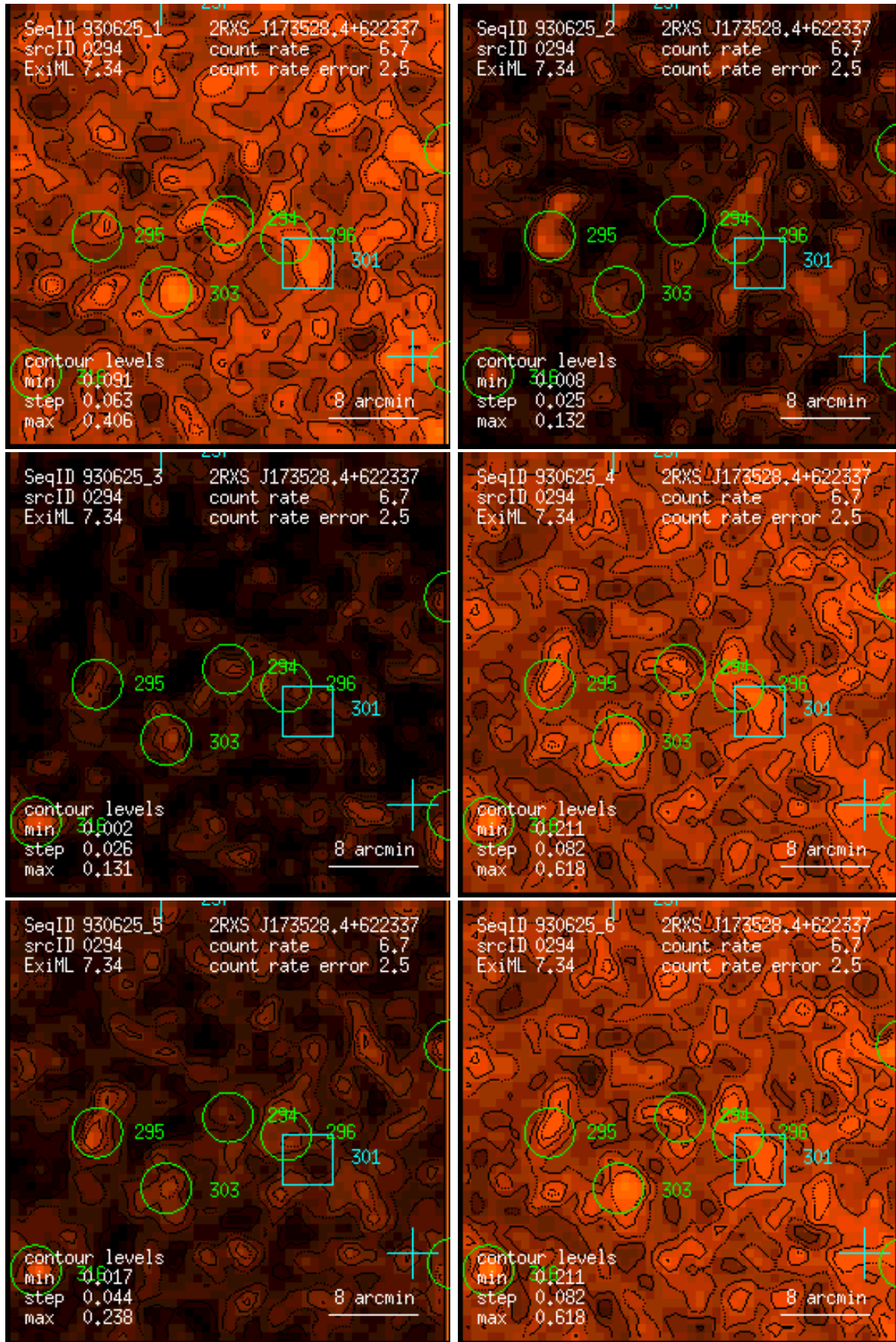
Figure 294: RASS 930625: detection 0294: band rate images, Gaussian filter: (1) PSPC channels 11 – 41, (2) 52 – 90, (3) 91 – 201, (4) 11 – 235, (5) 52 – 201, (6) 11 – 201. Broad band rates in counts/ks. Band rate contour levels in counts/ks/arcmin 2 .
