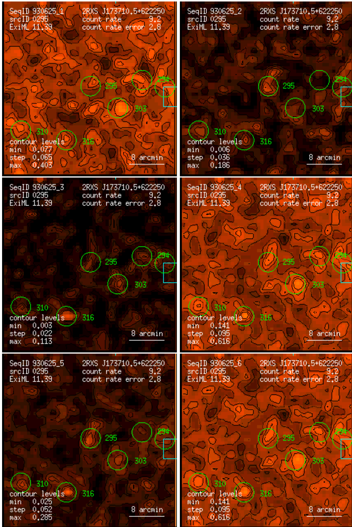
Figure 295: RASS 930625: detection 0295: band rate images, Gaussian filter: (1) PSPC channels 11 – 41, (2) 52 – 90, (3) 91 – 201, (4) 11 – 235, (5) 52 – 201, (6) 11 – 201. Broad band rates in counts/ks. Band rate contour levels in counts/ks/arcmin 2 .
