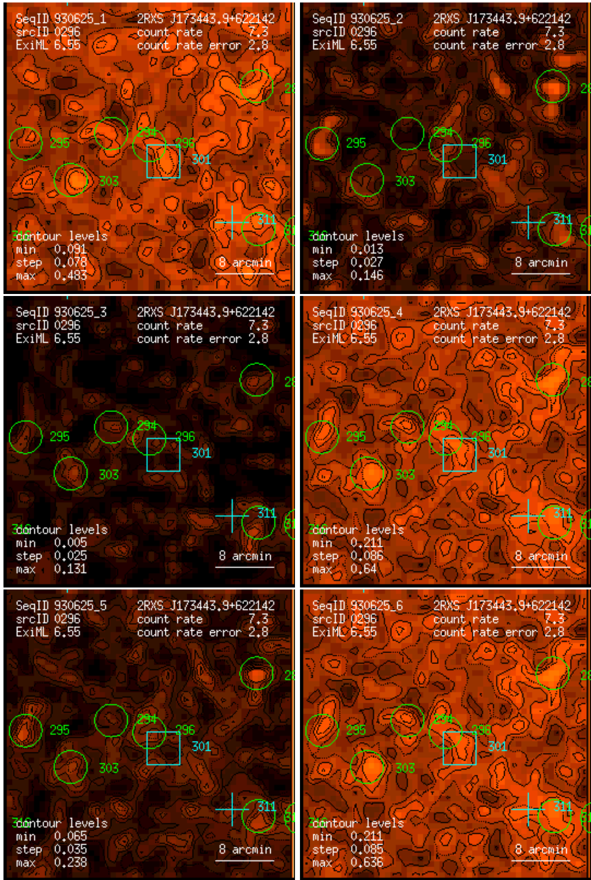
Figure 296: RASS 930625: detection 0296: band rate images, Gaussian filter: (1) PSPC channels 11 – 41, (2) 52 – 90, (3) 91 – 201, (4) 11 – 235, (5) 52 – 201, (6) 11 – 201. Broad band rates in counts/ks. Band rate contour levels in counts/ks/arcmin 2 .
