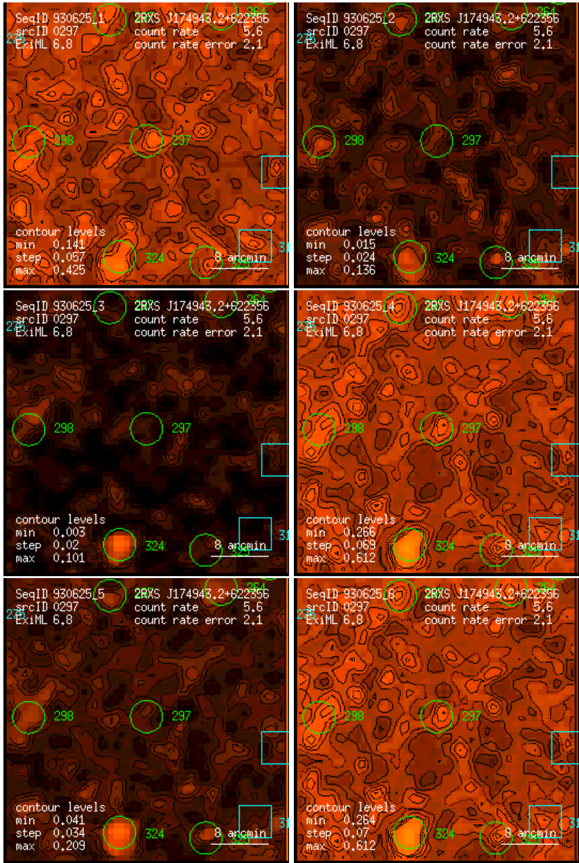
Figure 297: RASS 930625: detection 0297: band rate images, Gaussian filter: (1) PSPC channels 11 – 41, (2) 52 – 90, (3) 91 – 201, (4) 11 – 235, (5) 52 – 201, (6) 11 – 201. Broad band rates in counts/ks. Band rate contour levels in counts/ks/arcmin 2 .
