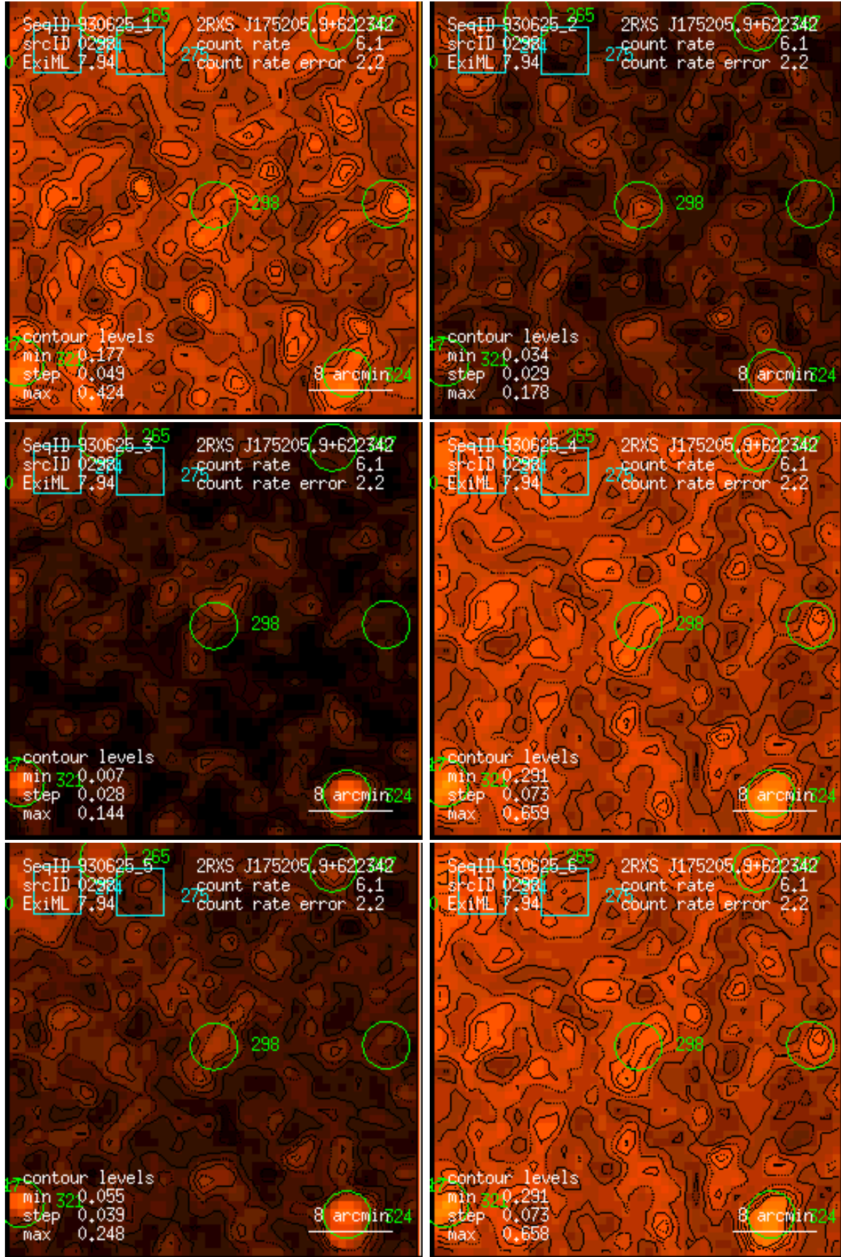
Figure 298: RASS 930625: detection 0298: band rate images, Gaussian filter: (1) PSPC channels 11 – 41, (2) 52 – 90, (3) 91 – 201, (4) 11 – 235, (5) 52 – 201, (6) 11 – 201. Broad band rates in counts/ks. Band rate contour levels in counts/ks/arcmin 2 .
