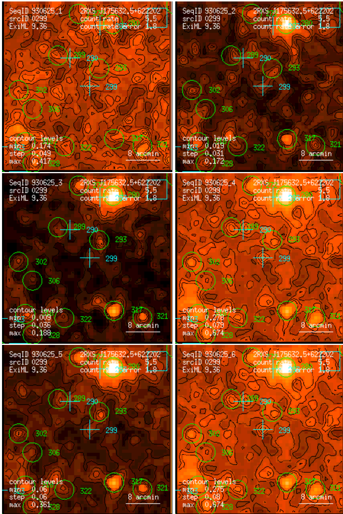
Figure 299: RASS 930625: detection 0299: band rate images, Gaussian filter: (1) PSPC channels 11 – 41, (2) 52 – 90, (3) 91 – 201, (4) 11 – 235, (5) 52 – 201, (6) 11 – 201. Broad band rates in counts/ks. Band rate contour levels in counts/ks/arcmin 2 .
