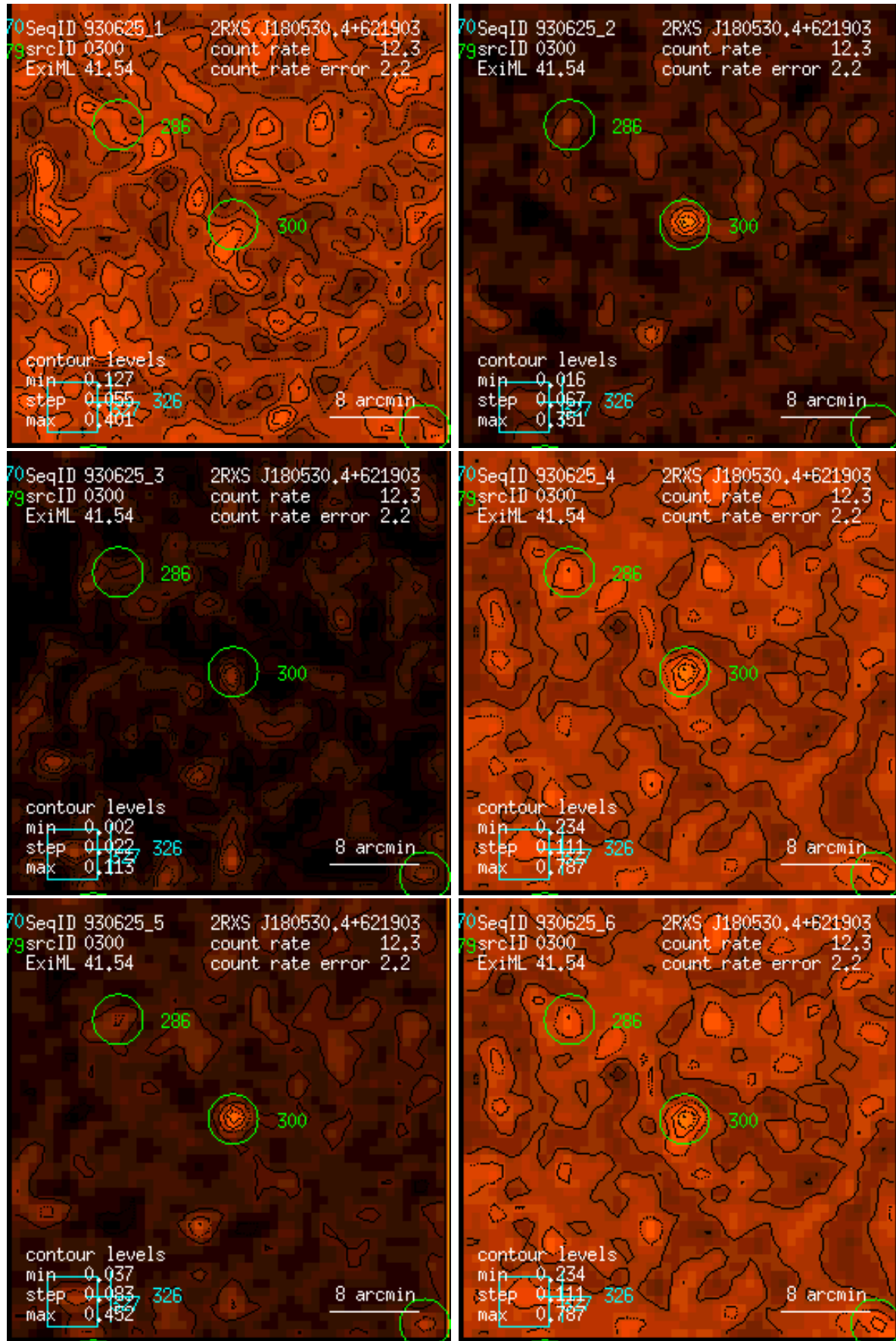
Figure 300: RASS 930625: detection 0300: band rate images, Gaussian filter: (1) PSPC channels 11 – 41, (2) 52 – 90, (3) 91 – 201, (4) 11 – 235, (5) 52 – 201, (6) 11 – 201. Broad band rates in counts/ks. Band rate contour levels in counts/ks/arcmin 2 .
