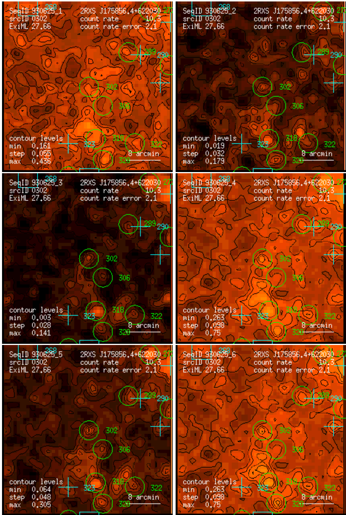
Figure 302: RASS 930625: detection 0302: band rate images, Gaussian filter: (1) PSPC channels 11 – 41, (2) 52 – 90, (3) 91 – 201, (4) 11 – 235, (5) 52 – 201, (6) 11 – 201. Broad band rates in counts/ks. Band rate contour levels in counts/ks/arcmin 2 .
