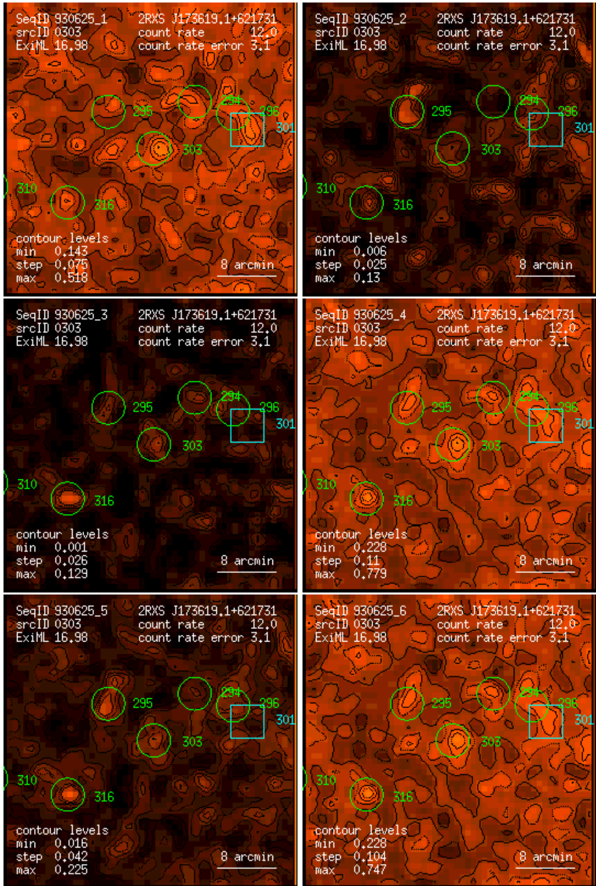
Figure 303: RASS 930625: detection 0303: band rate images, Gaussian filter: (1) PSPC channels 11 – 41, (2) 52 – 90, (3) 91 – 201, (4) 11 – 235, (5) 52 – 201, (6) 11 – 201. Broad band rates in counts/ks. Band rate contour levels in counts/ks/arcmin 2 .
