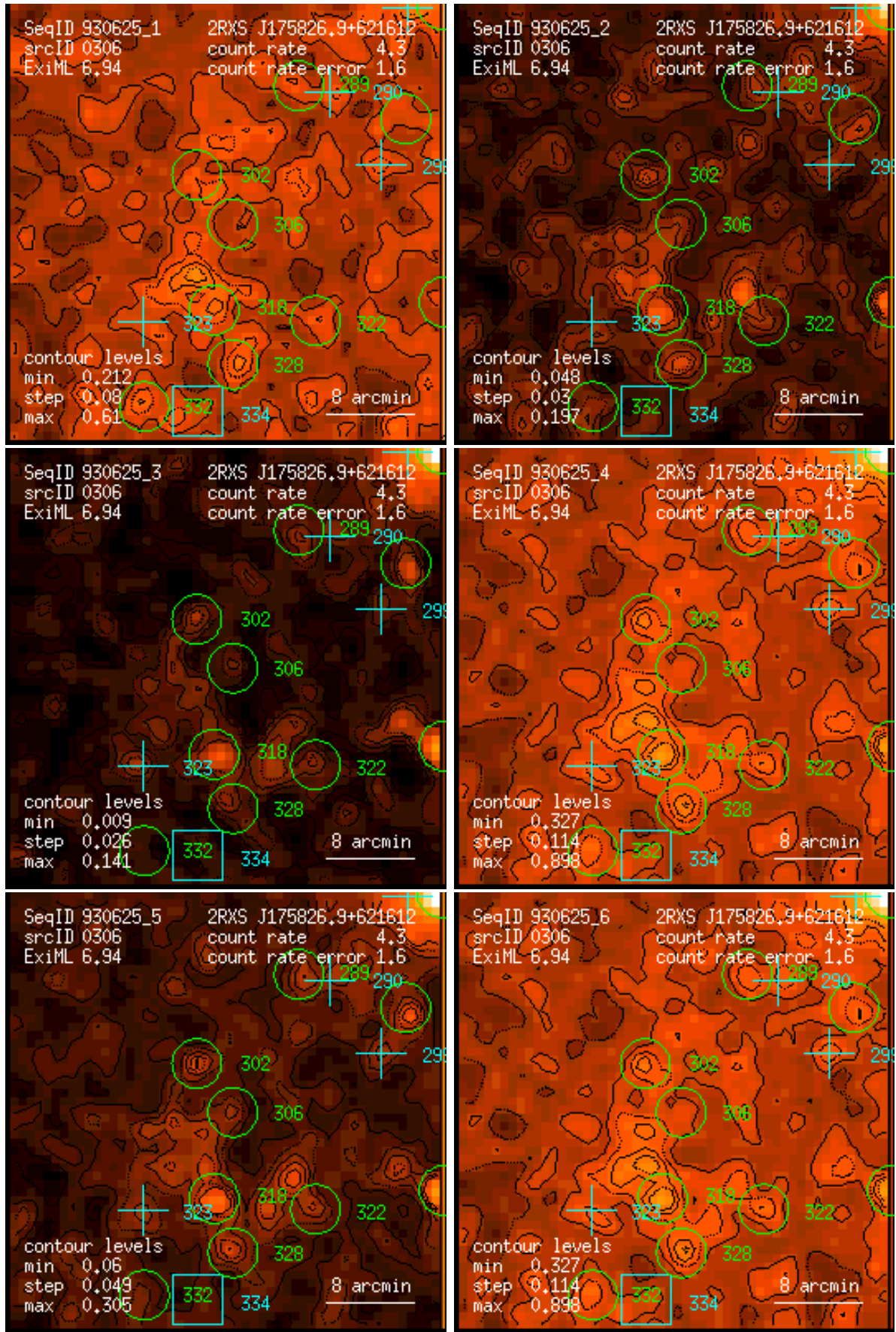
Figure 306: RASS 930625: detection 0306: band rate images, Gaussian filter: (1) PSPC channels 11 – 41, (2) 52 – 90, (3) 91 – 201, (4) 11 – 235, (5) 52 – 201, (6) 11 – 201. Broad band rates in counts/ks. Band rate contour levels in counts/ks/arcmin 2 .
