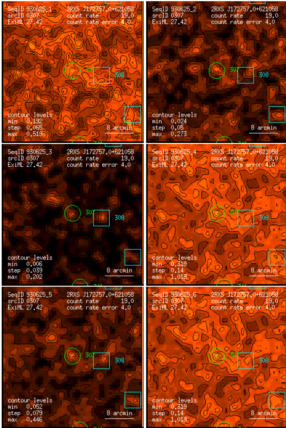
Figure 307: RASS 930625: detection 0307: band rate images, Gaussian filter: (1) PSPC channels 11 – 41, (2) 52 – 90, (3) 91 – 201, (4) 11 – 235, (5) 52 – 201, (6) 11 – 201. Broad band rates in counts/ks. Band rate contour levels in counts/ks/arcmin 2 .
