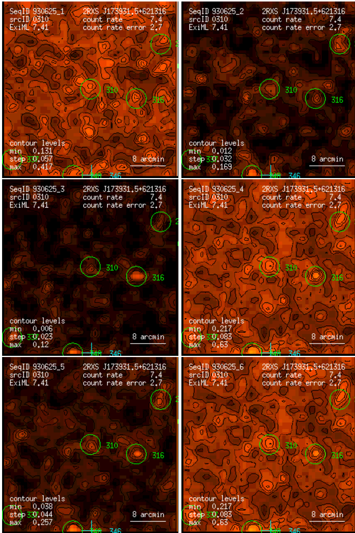
Figure 310: RASS 930625: detection 0310: band rate images, Gaussian filter: (1) PSPC channels 11 – 41, (2) 52 – 90, (3) 91 – 201, (4) 11 – 235, (5) 52 – 201, (6) 11 – 201. Broad band rates in counts/ks. Band rate contour levels in counts/ks/arcmin 2 .
