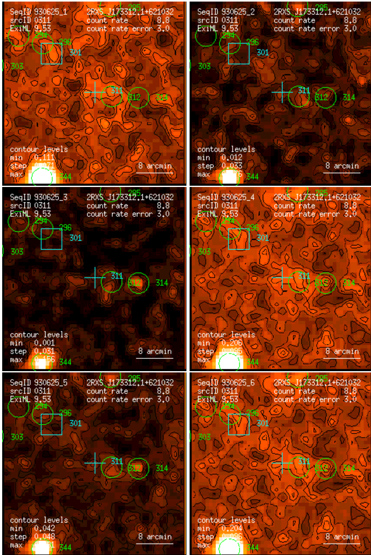
Figure 311: RASS 930625: detection 0311: band rate images, Gaussian filter: (1) PSPC channels 11 – 41, (2) 52 – 90, (3) 91 – 201, (4) 11 – 235, (5) 52 – 201, (6) 11 – 201. Broad band rates in counts/ks. Band rate contour levels in counts/ks/arcmin 2 .
