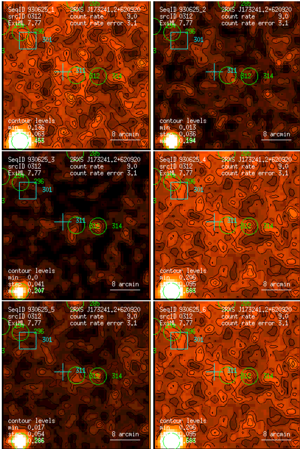
Figure 312: RASS 930625: detection 0312: band rate images, Gaussian filter: (1) PSPC channels 11 – 41, (2) 52 – 90, (3) 91 – 201, (4) 11 – 235, (5) 52 – 201, (6) 11 – 201. Broad band rates in counts/ks. Band rate contour levels in counts/ks/arcmin 2 .
