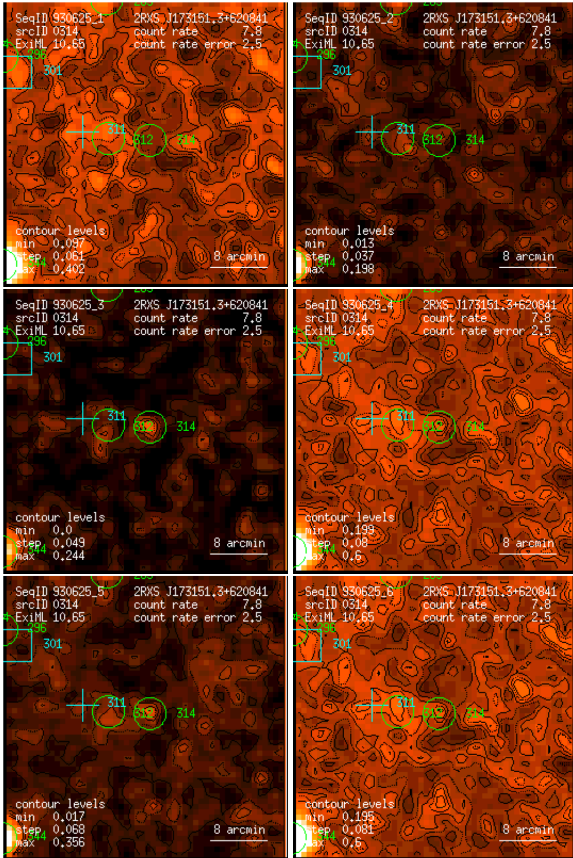
Figure 314: RASS 930625: detection 0314: band rate images, Gaussian filter: (1) PSPC channels 11 – 41, (2) 52 – 90, (3) 91 – 201, (4) 11 – 235, (5) 52 – 201, (6) 11 – 201. Broad band rates in counts/ks. Band rate contour levels in counts/ks/arcmin 2 .
