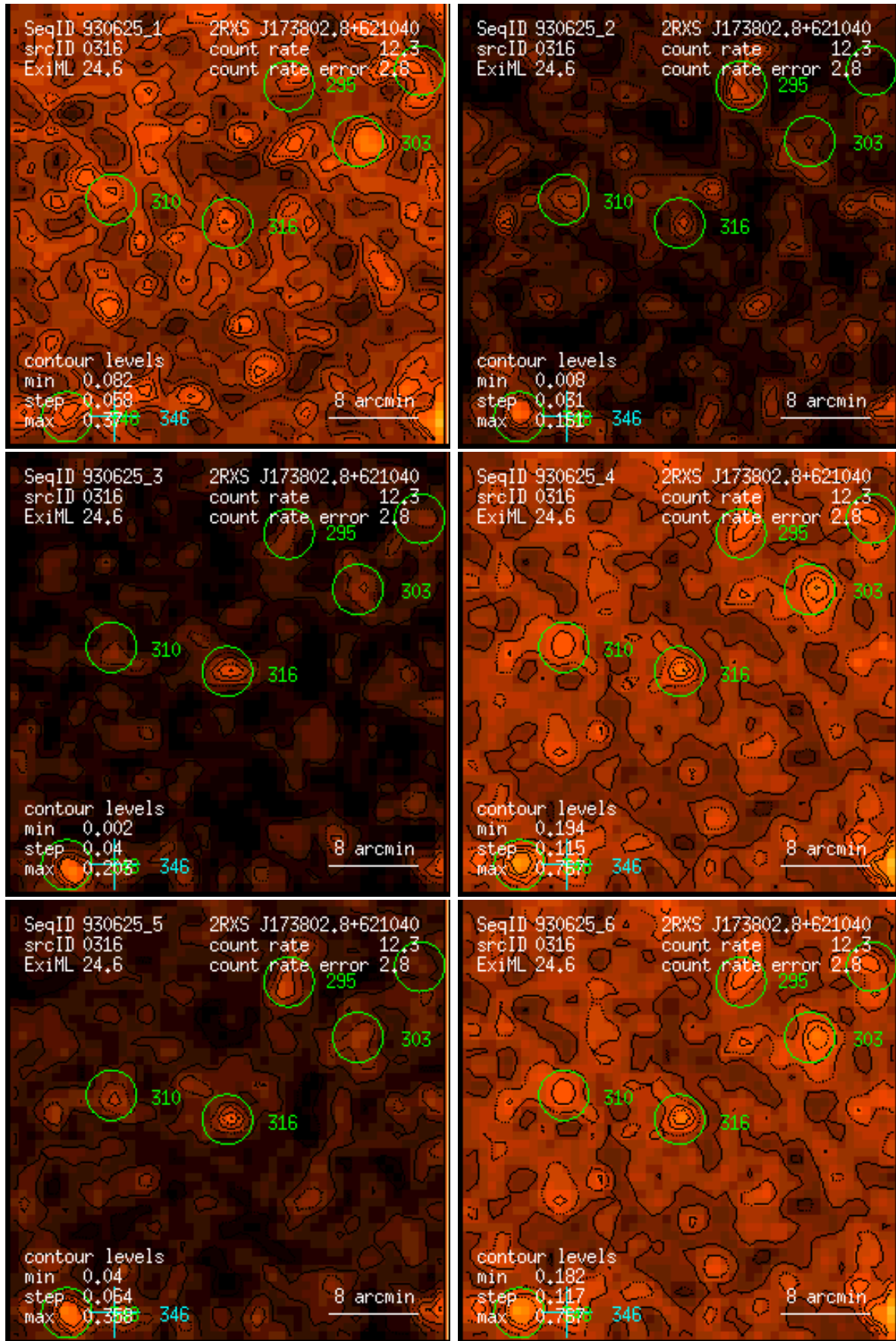
Figure 316: RASS 930625: detection 0316: band rate images, Gaussian filter: (1) PSPC channels 11 – 41, (2) 52 – 90, (3) 91 – 201, (4) 11 – 235, (5) 52 – 201, (6) 11 – 201. Broad band rates in counts/ks. Band rate contour levels in counts/ks/arcmin 2 .
