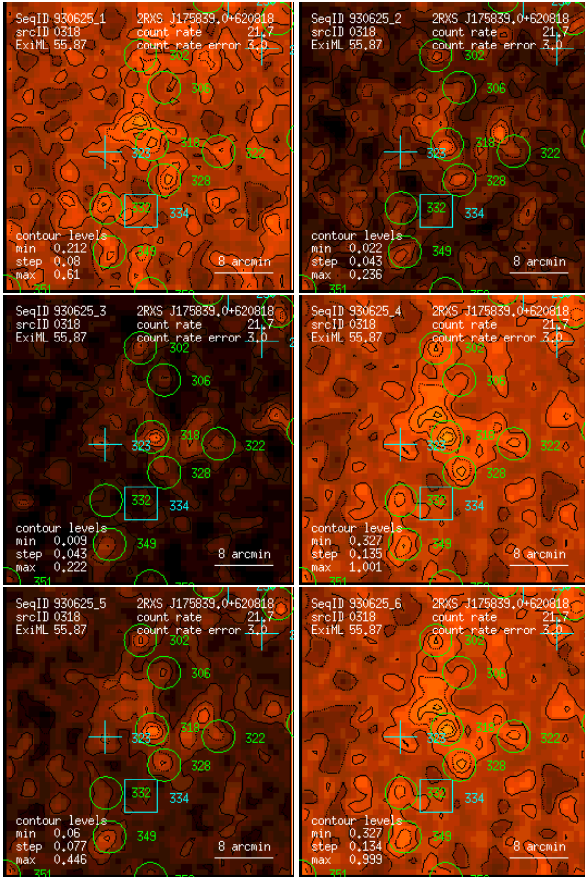
Figure 318: RASS 930625: detection 0318: band rate images, Gaussian filter: (1) PSPC channels 11 – 41, (2) 52 – 90, (3) 91 – 201, (4) 11 – 235, (5) 52 – 201, (6) 11 – 201. Broad band rates in counts/ks. Band rate contour levels in counts/ks/arcmin 2 .
