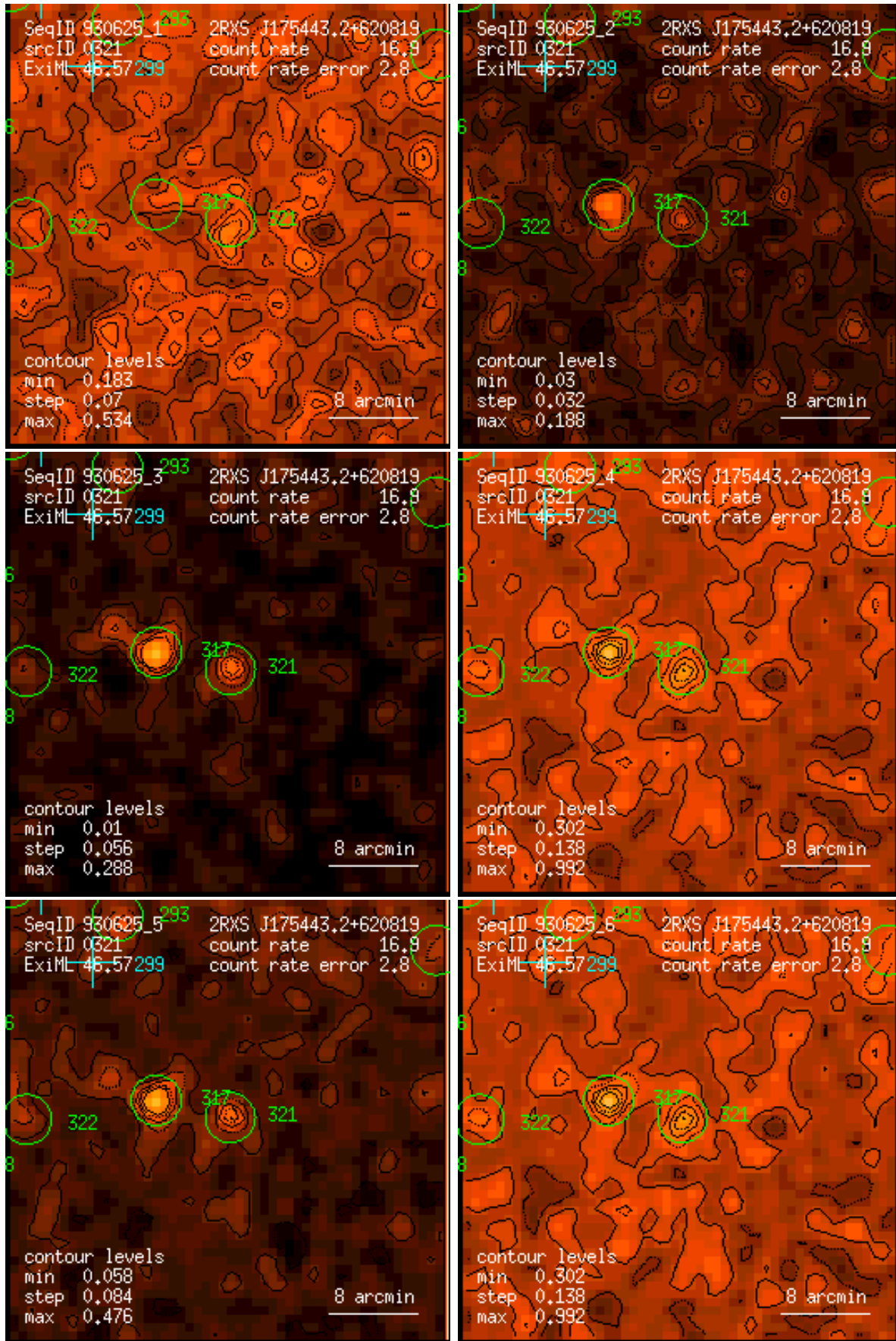
Figure 321: RASS 930625: detection 0321: band rate images, Gaussian filter: (1) PSPC channels 11 – 41, (2) 52 – 90, (3) 91 – 201, (4) 11 – 235, (5) 52 – 201, (6) 11 – 201. Broad band rates in counts/ks. Band rate contour levels in counts/ks/arcmin 2 .
