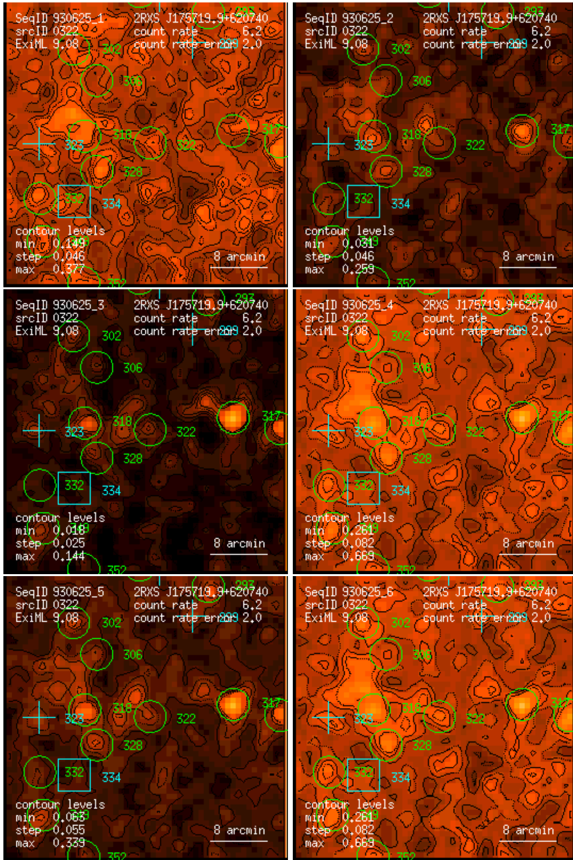
Figure 322: RASS 930625: detection 0322: band rate images, Gaussian filter: (1) PSPC channels 11 – 41, (2) 52 – 90, (3) 91 – 201, (4) 11 – 235, (5) 52 – 201, (6) 11 – 201. Broad band rates in counts/ks. Band rate contour levels in counts/ks/arcmin 2 .
