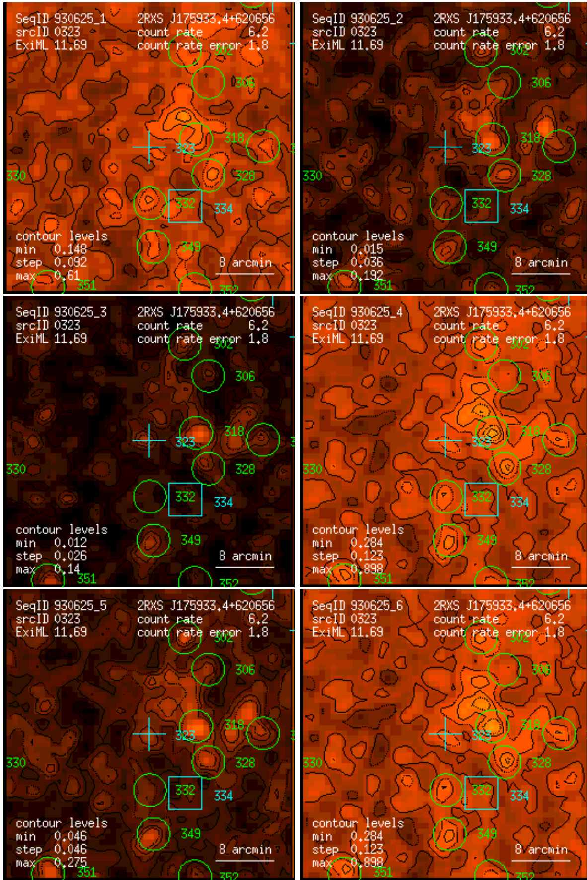
Figure 323: RASS 930625: detection 0323: band rate images, Gaussian filter: (1) PSPC channels 11 – 41, (2) 52 – 90, (3) 91 – 201, (4) 11 – 235, (5) 52 – 201, (6) 11 – 201. Broad band rates in counts/ks. Band rate contour levels in counts/ks/arcmin 2 .
