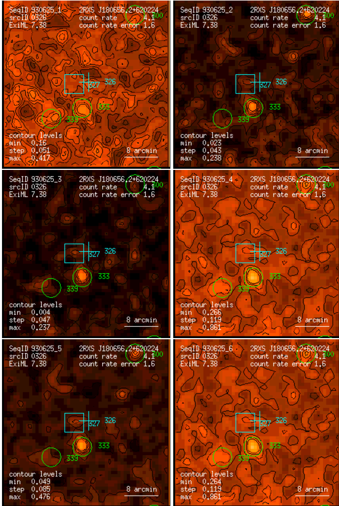
Figure 326: RASS 930625: detection 0326: band rate images, Gaussian filter: (1) PSPC channels 11 – 41, (2) 52 – 90, (3) 91 – 201, (4) 11 – 235, (5) 52 – 201, (6) 11 – 201. Broad band rates in counts/ks. Band rate contour levels in counts/ks/arcmin 2 .
