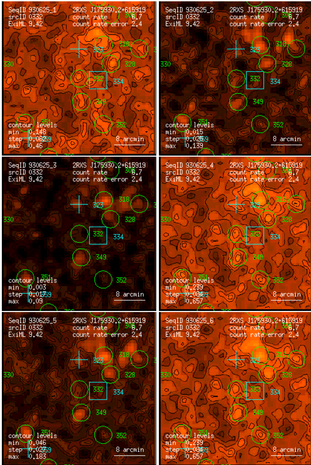
Figure 332: RASS 930625: detection 0332: band rate images, Gaussian filter: (1) PSPC channels 11 – 41, (2) 52 – 90, (3) 91 – 201, (4) 11 – 235, (5) 52 – 201, (6) 11 – 201. Broad band rates in counts/ks. Band rate contour levels in counts/ks/arcmin 2 .
