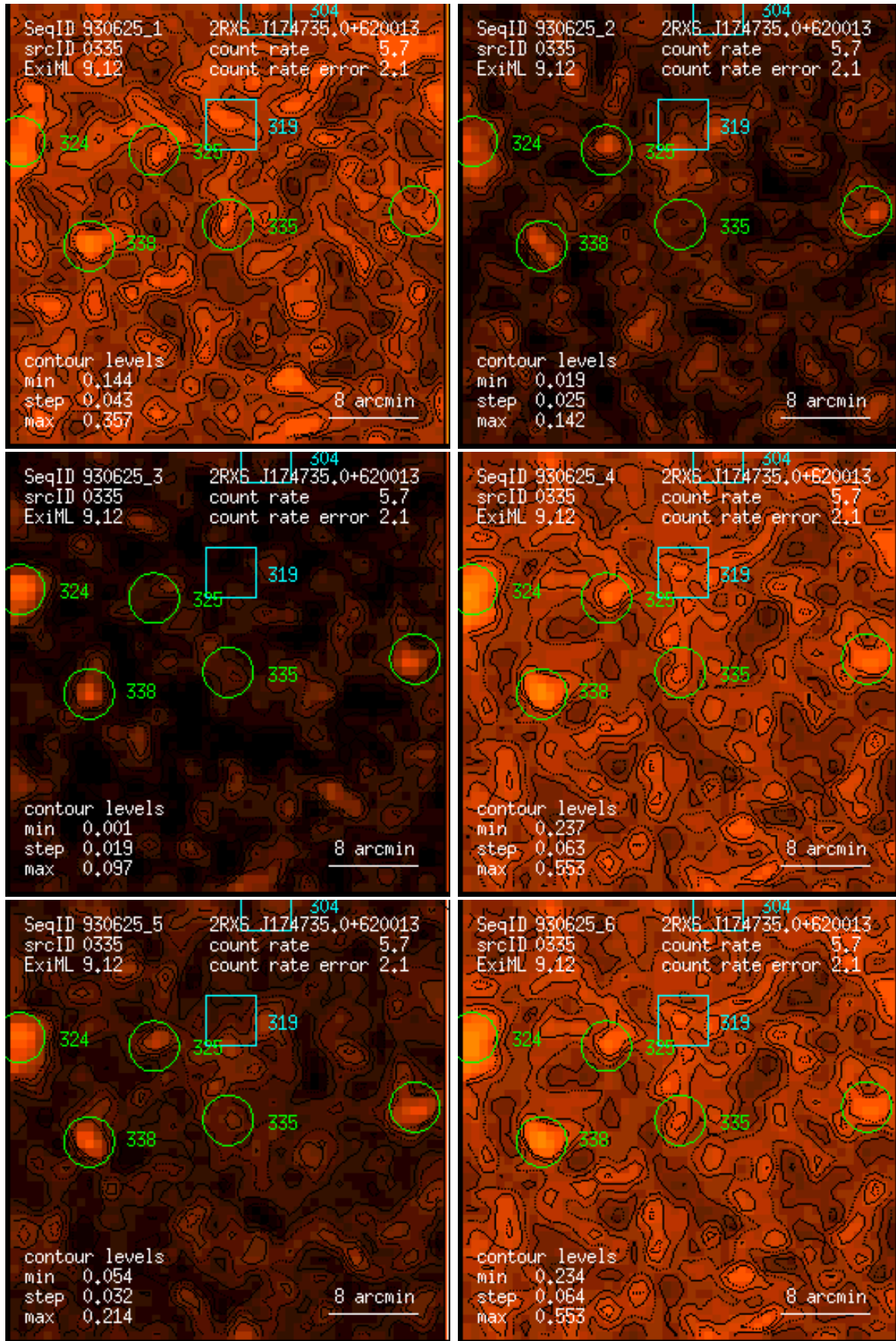
Figure 335: RASS 930625: detection 0335: band rate images, Gaussian filter: (1) PSPC channels 11 – 41, (2) 52 – 90, (3) 91 – 201, (4) 11 – 235, (5) 52 – 201, (6) 11 – 201. Broad band rates in counts/ks. Band rate contour levels in counts/ks/arcmin 2 .
