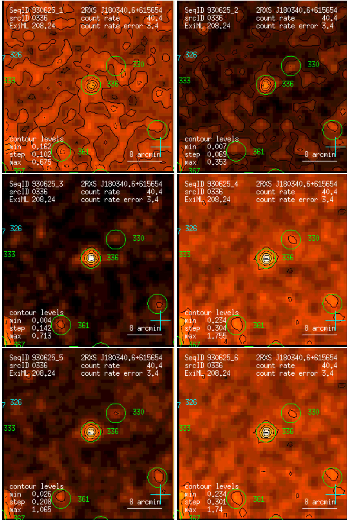
Figure 336: RASS 930625: detection 0336: band rate images, Gaussian filter: (1) PSPC channels 11 – 41, (2) 52 – 90, (3) 91 – 201, (4) 11 – 235, (5) 52 – 201, (6) 11 – 201. Broad band rates in counts/ks. Band rate contour levels in counts/ks/arcmin 2 .
