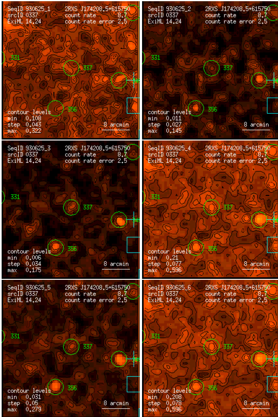
Figure 337: RASS 930625: detection 0337: band rate images, Gaussian filter: (1) PSPC channels 11 – 41, (2) 52 – 90, (3) 91 – 201, (4) 11 – 235, (5) 52 – 201, (6) 11 – 201. Broad band rates in counts/ks. Band rate contour levels in counts/ks/arcmin 2 .
