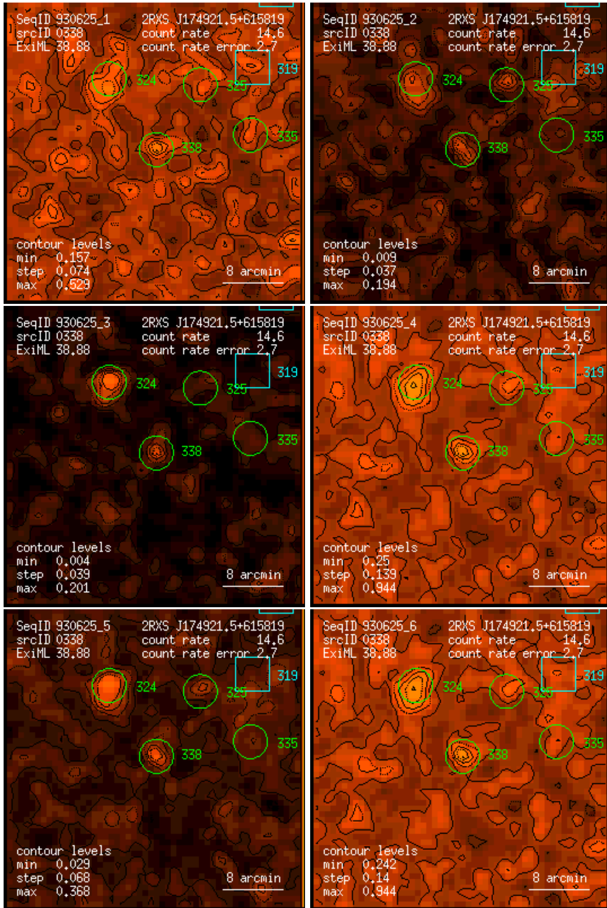
Figure 338: RASS 930625: detection 0338: band rate images, Gaussian filter: (1) PSPC channels 11 – 41, (2) 52 – 90, (3) 91 – 201, (4) 11 – 235, (5) 52 – 201, (6) 11 – 201. Broad band rates in counts/ks. Band rate contour levels in counts/ks/arcmin 2 .
