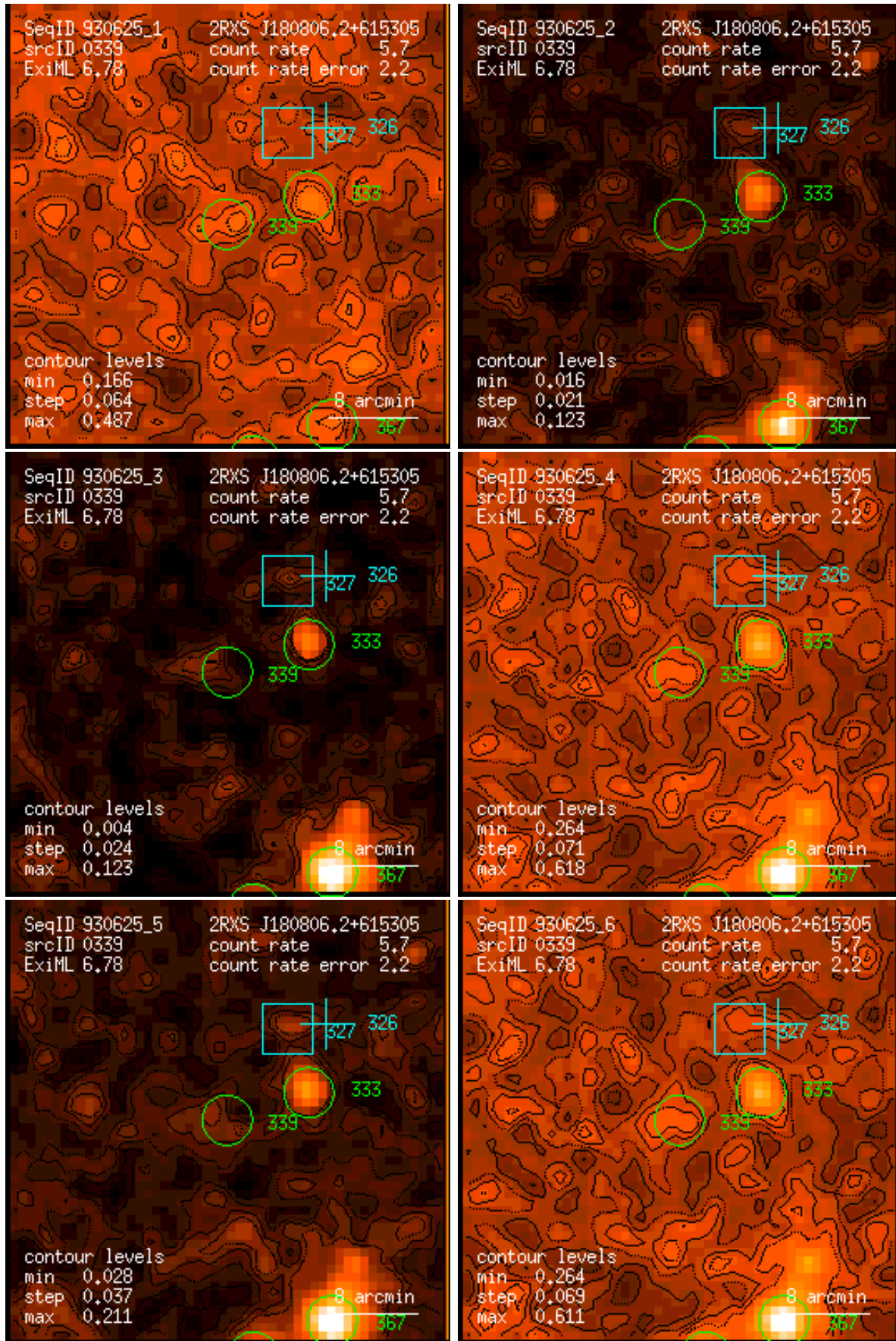
Figure 339: RASS 930625: detection 0339: band rate images, Gaussian filter: (1) PSPC channels 11 – 41, (2) 52 – 90, (3) 91 – 201, (4) 11 – 235, (5) 52 – 201, (6) 11 – 201. Broad band rates in counts/ks. Band rate contour levels in counts/ks/arcmin 2 .
