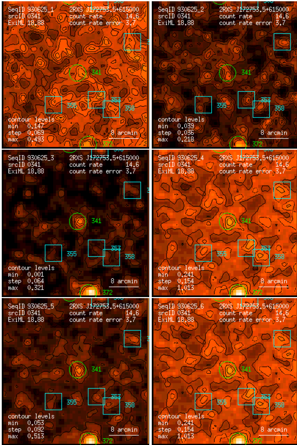
Figure 341: RASS 930625: detection 0341: band rate images, Gaussian filter: (1) PSPC channels 11 – 41, (2) 52 – 90, (3) 91 – 201, (4) 11 – 235, (5) 52 – 201, (6) 11 – 201. Broad band rates in counts/ks. Band rate contour levels in counts/ks/arcmin 2 .
