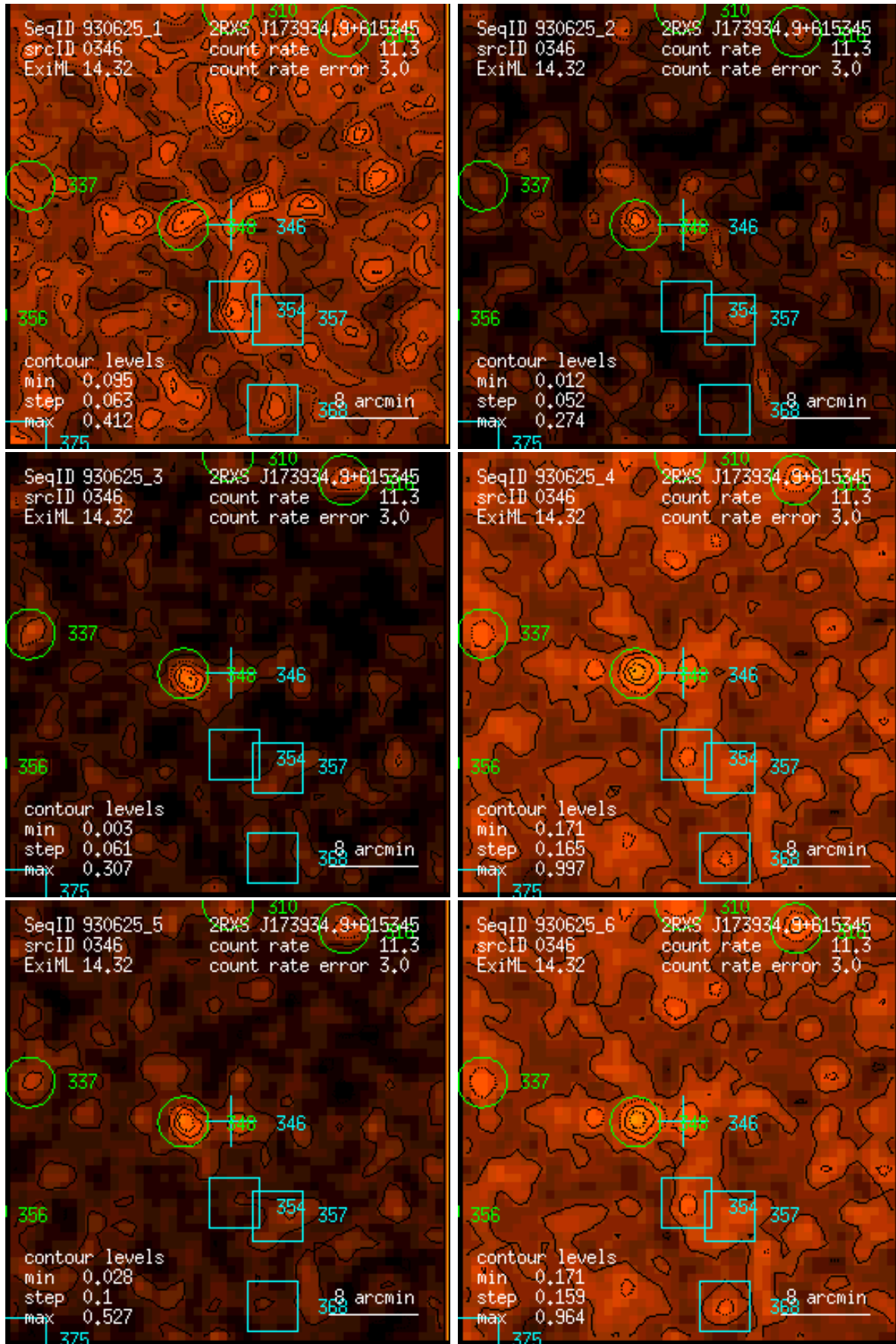
Figure 346: RASS 930625: detection 0346: band rate images, Gaussian filter: (1) PSPC channels 11 – 41, (2) 52 – 90, (3) 91 – 201, (4) 11 – 235, (5) 52 – 201, (6) 11 – 201. Broad band rates in counts/ks. Band rate contour levels in counts/ks/arcmin 2 .
