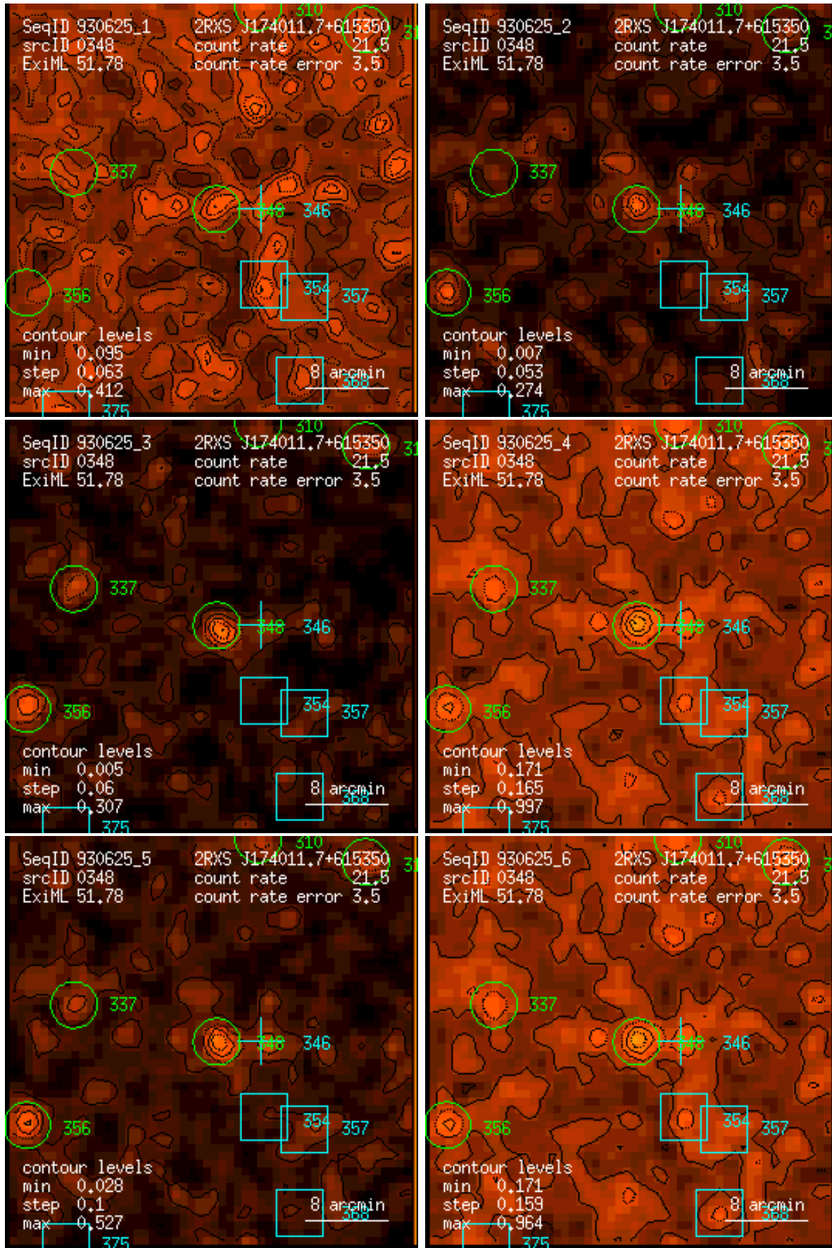
Figure 348: RASS 930625: detection 0348: band rate images, Gaussian filter: (1) PSPC channels 11 – 41, (2) 52 – 90, (3) 91 – 201, (4) 11 – 235, (5) 52 – 201, (6) 11 – 201. Broad band rates in counts/ks. Band rate contour levels in counts/ks/arcmin 2 .
