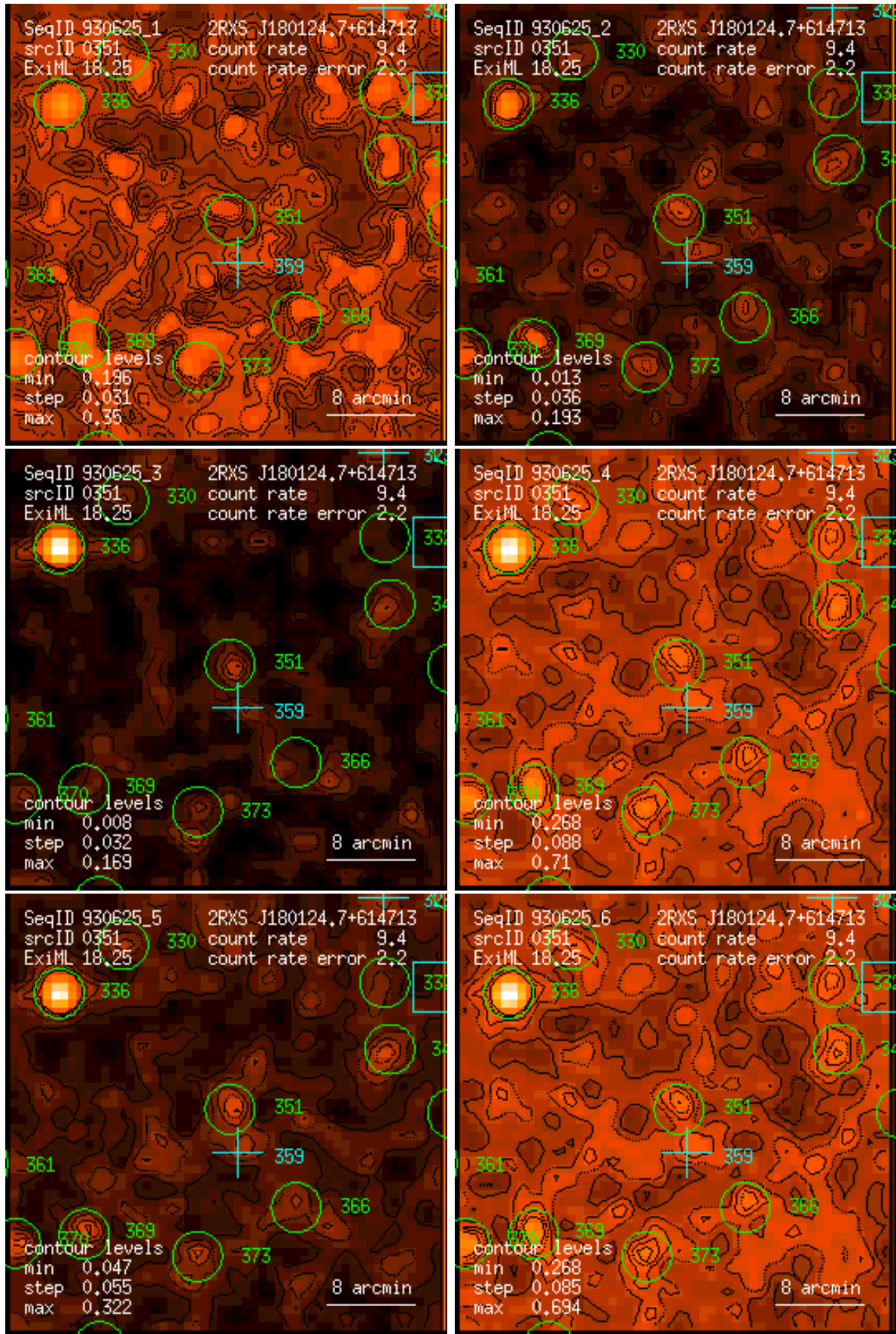
Figure 351: RASS 930625: detection 0351: band rate images, Gaussian filter: (1) PSPC channels 11 – 41, (2) 52 – 90, (3) 91 – 201, (4) 11 – 235, (5) 52 – 201, (6) 11 – 201. Broad band rates in counts/ks. Band rate contour levels in counts/ks/arcmin 2 .
