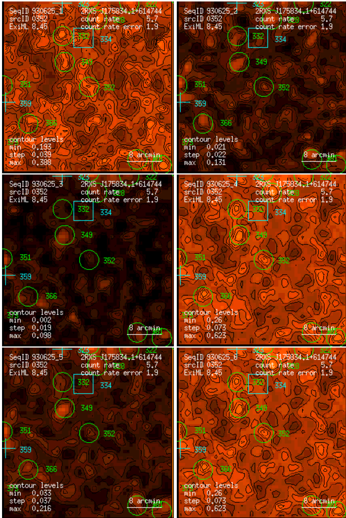
Figure 352: RASS 930625: detection 0352: band rate images, Gaussian filter: (1) PSPC channels 11 – 41, (2) 52 – 90, (3) 91 – 201, (4) 11 – 235, (5) 52 – 201, (6) 11 – 201. Broad band rates in counts/ks. Band rate contour levels in counts/ks/arcmin 2 .
