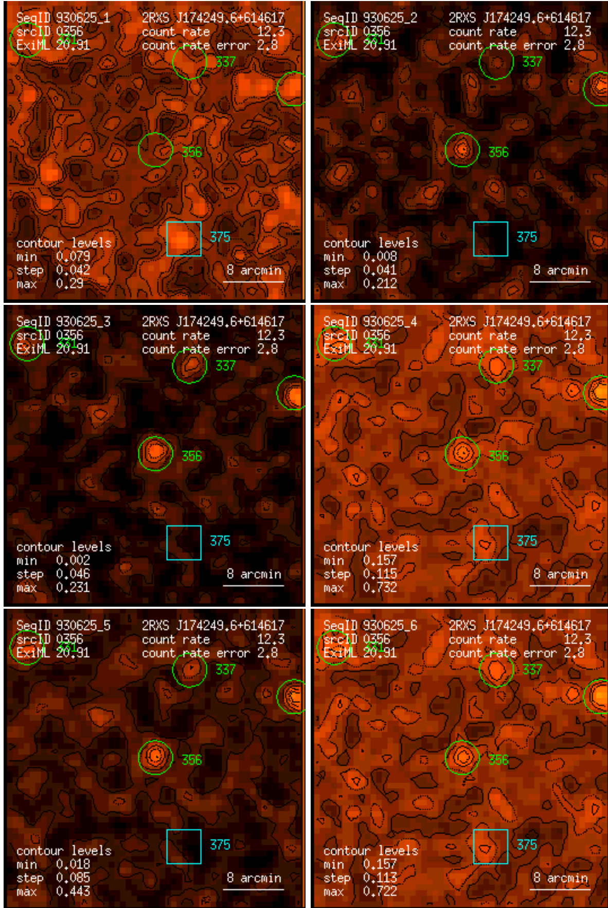
Figure 356: RASS 930625: detection 0356: band rate images, Gaussian filter: (1) PSPC channels 11 – 41, (2) 52 – 90, (3) 91 – 201, (4) 11 – 235, (5) 52 – 201, (6) 11 – 201. Broad band rates in counts/ks. Band rate contour levels in counts/ks/arcmin 2 .
