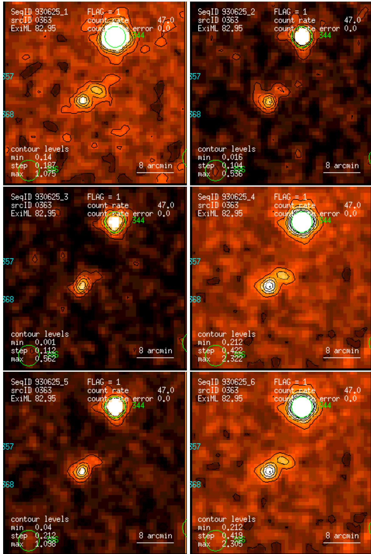
Figure 363: RASS 930625: detection 0363: band rate images, Gaussian filter: (1) PSPC channels 11 – 41, (2) 52 – 90, (3) 91 – 201, (4) 11 – 235, (5) 52 – 201, (6) 11 – 201. Broad band rates in counts/ks. Band rate contour levels in counts/ks/arcmin 2 .
