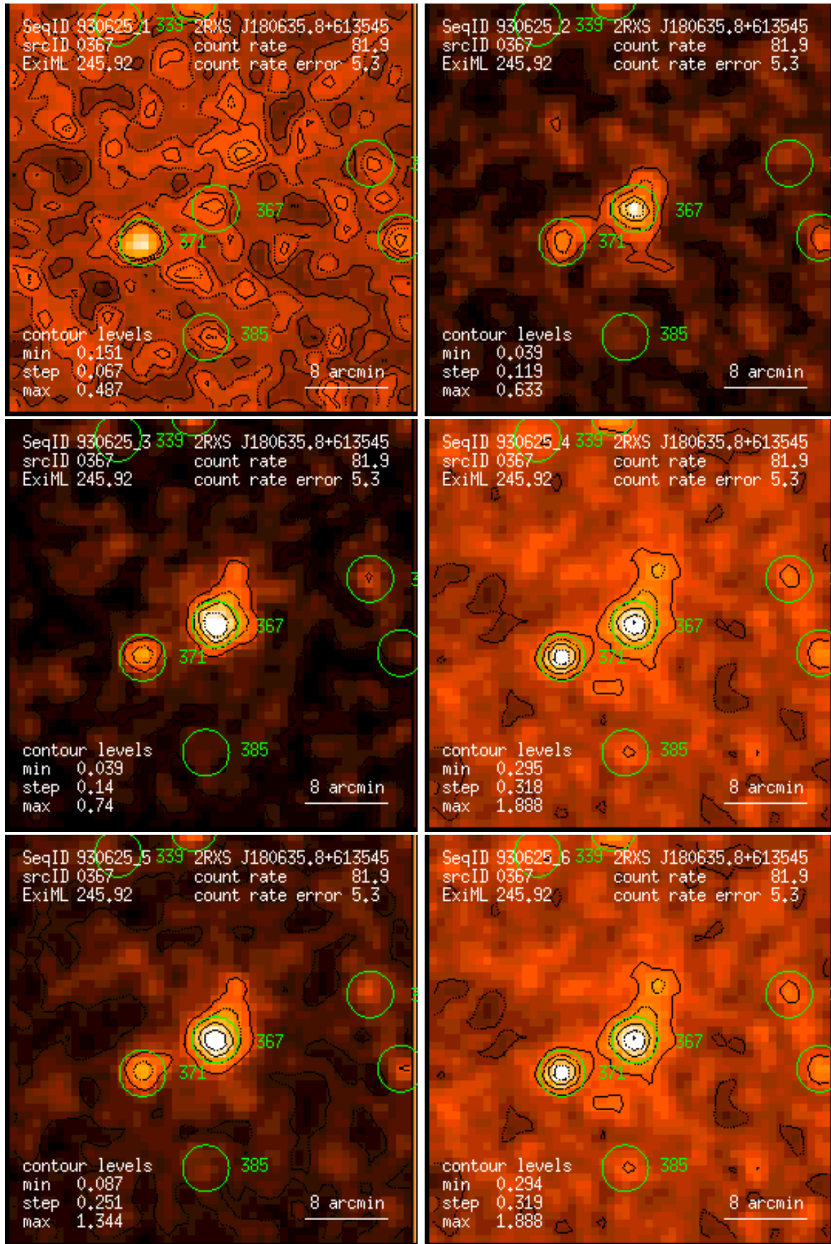
Figure 367: RASS 930625: detection 0367: band rate images, Gaussian filter: (1) PSPC channels 11 – 41, (2) 52 – 90, (3) 91 – 201, (4) 11 – 235, (5) 52 – 201, (6) 11 – 201. Broad band rates in counts/ks. Band rate contour levels in counts/ks/arcmin 2 .
