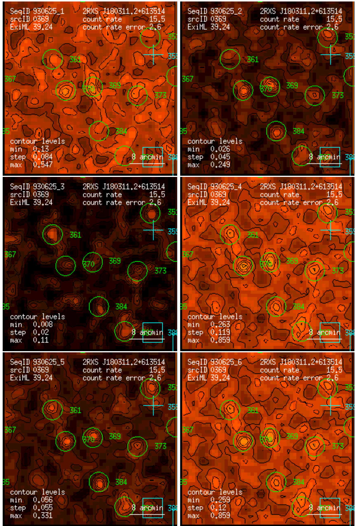
Figure 369: RASS 930625: detection 0369: band rate images, Gaussian filter: (1) PSPC channels 11 – 41, (2) 52 – 90, (3) 91 – 201, (4) 11 – 235, (5) 52 – 201, (6) 11 – 201. Broad band rates in counts/ks. Band rate contour levels in counts/ks/arcmin 2 .
