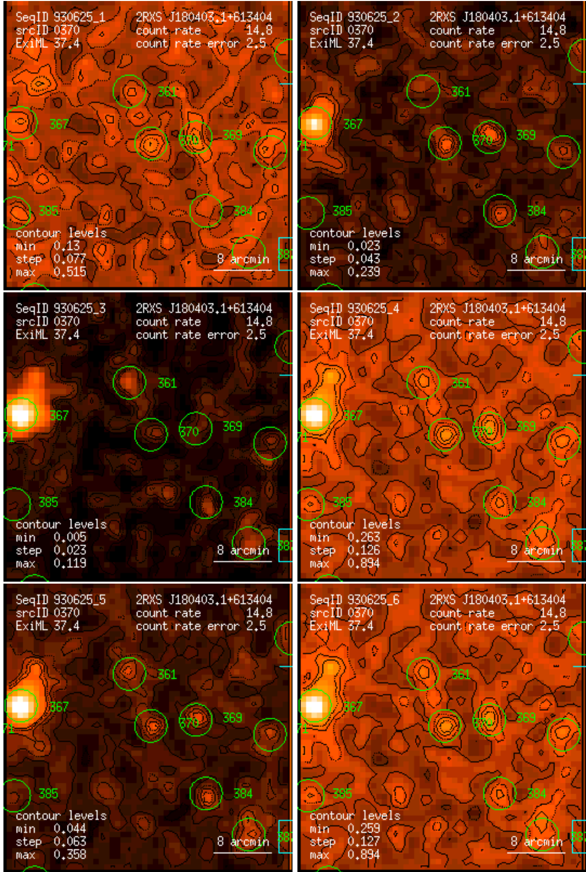
Figure 370: RASS 930625: detection 0370: band rate images, Gaussian filter: (1) PSPPC channels 11 – 41, (2) 52 – 90, (3) 91 – 201, (4) 11 – 235, (5) 52 – 201, (6) 11 – 201. Broad band rates in counts/ks. Band rate contour levels in counts/ks/arcmin 2 .
