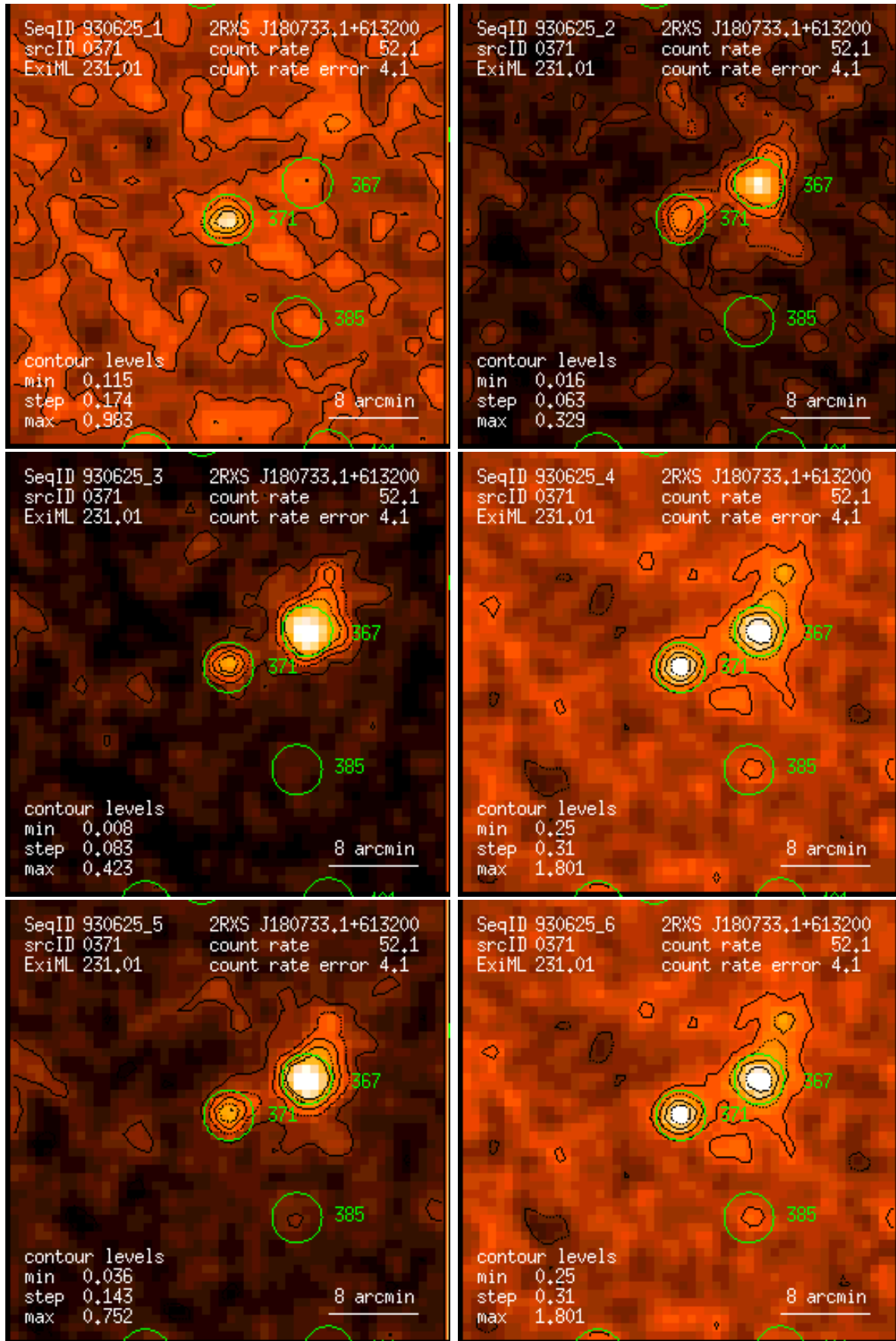
Figure 371: RASS 930625: detection 0371: band rate images, Gaussian filter: (1) PSPC channels 11 – 41, (2) 52 – 90, (3) 91 – 201, (4) 11 – 235, (5) 52 – 201, (6) 11 – 201. Broad band rates in counts/ks. Band rate contour levels in counts/ks/arcmin 2 .
