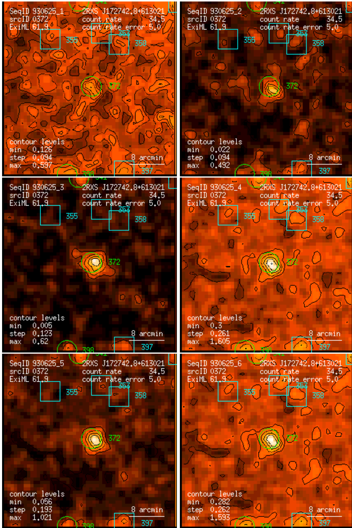
Figure 372: RASS 930625: detection 0372: band rate images, Gaussian filter: (1) PSPC channels 11 – 41, (2) 52 – 90, (3) 91 – 201, (4) 11 – 235, (5) 52 – 201, (6) 11 – 201. Broad band rates in counts/ks. Band rate contour levels in counts/ks/arcmin 2 .
