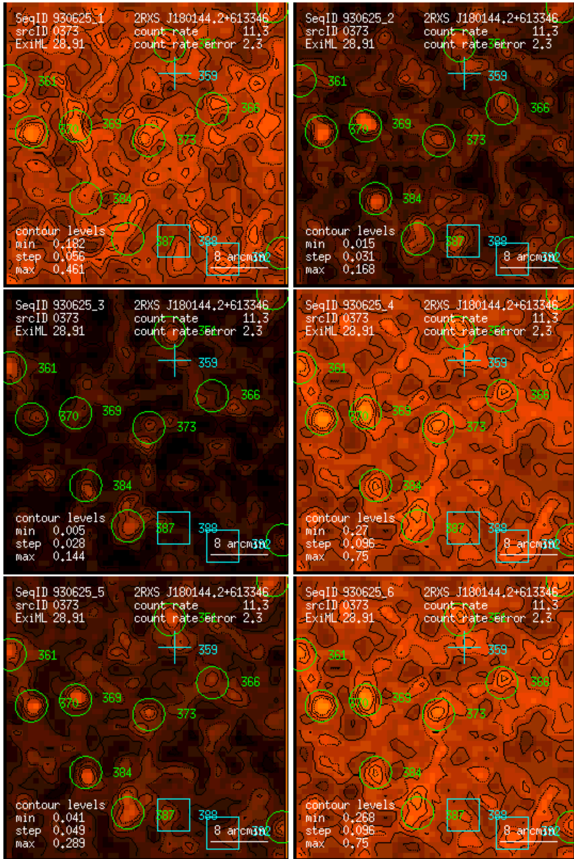
Figure 373: RASS 930625: detection 0373: band rate images, Gaussian filter: (1) PSPC channels 11 – 41, (2) 52 – 90, (3) 91 – 201, (4) 11 – 235, (5) 52 – 201, (6) 11 – 201. Broad band rates in counts/ks. Band rate contour levels in counts/ks/arcmin 2 .
