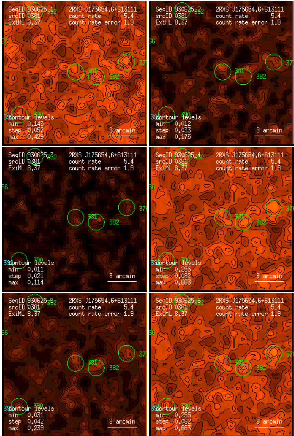
Figure 381: RASS 930625: detection 0381: band rate images, Gaussian filter: (1) PSPC channels 11 – 41, (2) 52 – 90, (3) 91 – 201, (4) 11 – 235, (5) 52 – 201, (6) 11 – 201. Broad band rates in counts/ks. Band rate contour levels in counts/ks/arcmin 2 .
