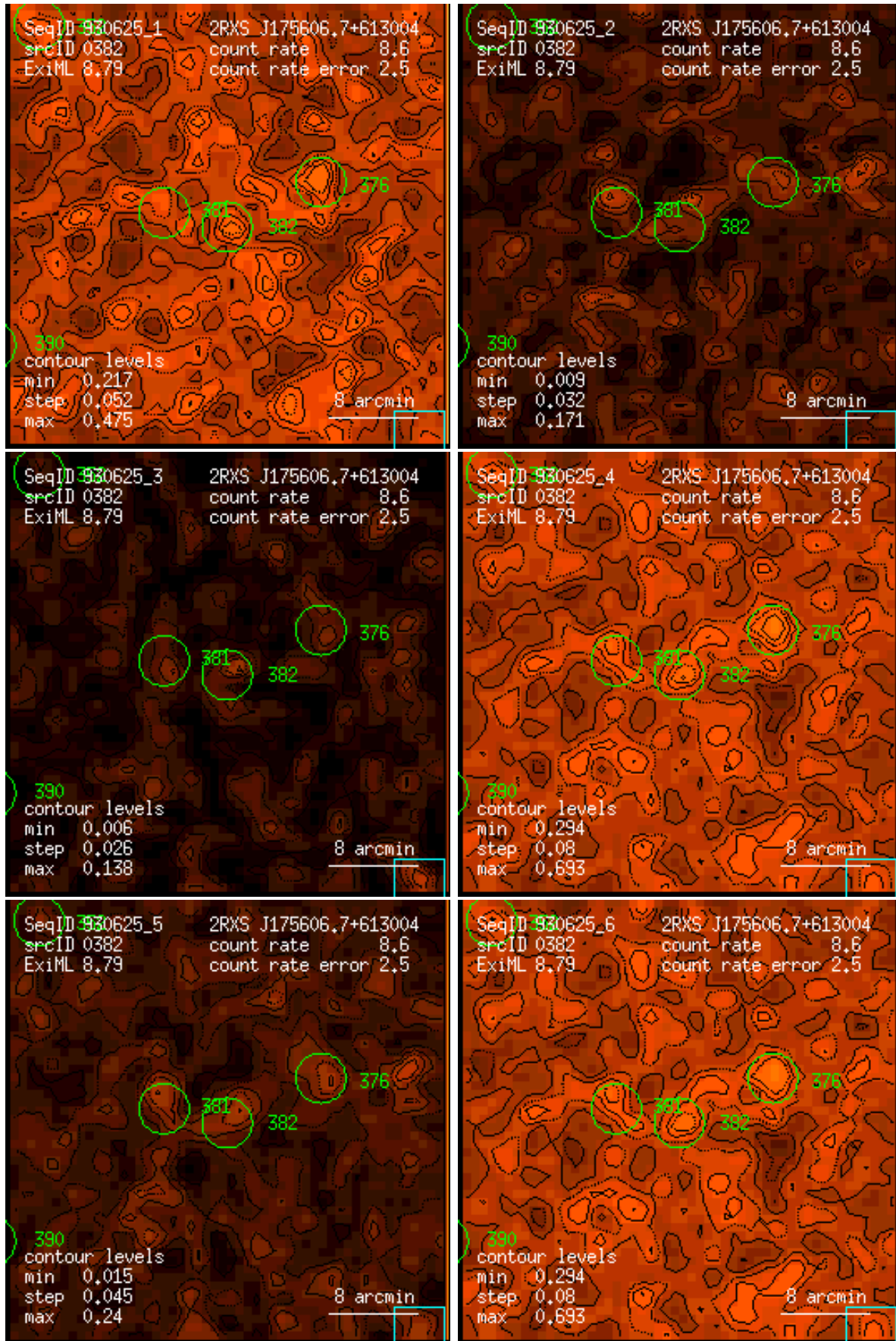
Figure 382: RASS 930625: detection 0382: band rate images, Gaussian filter: (1) PSPC channels 11 – 41, (2) 52 – 90, (3) 91 – 201, (4) 11 – 235, (5) 52 – 201, (6) 11 – 201. Broad band rates in counts/ks. Band rate contour levels in counts/ks/arcmin 2 .
