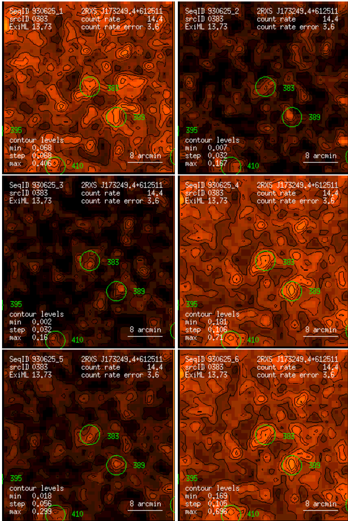
Figure 383: RASS 930625: detection 0383: band rate images, Gaussian filter: (1) PSPC channels 11 – 41, (2) 52 – 90, (3) 91 – 201, (4) 11 – 235, (5) 52 – 201, (6) 11 – 201. Broad band rates in counts/ks. Band rate contour levels in counts/ks/arcmin 2 .
