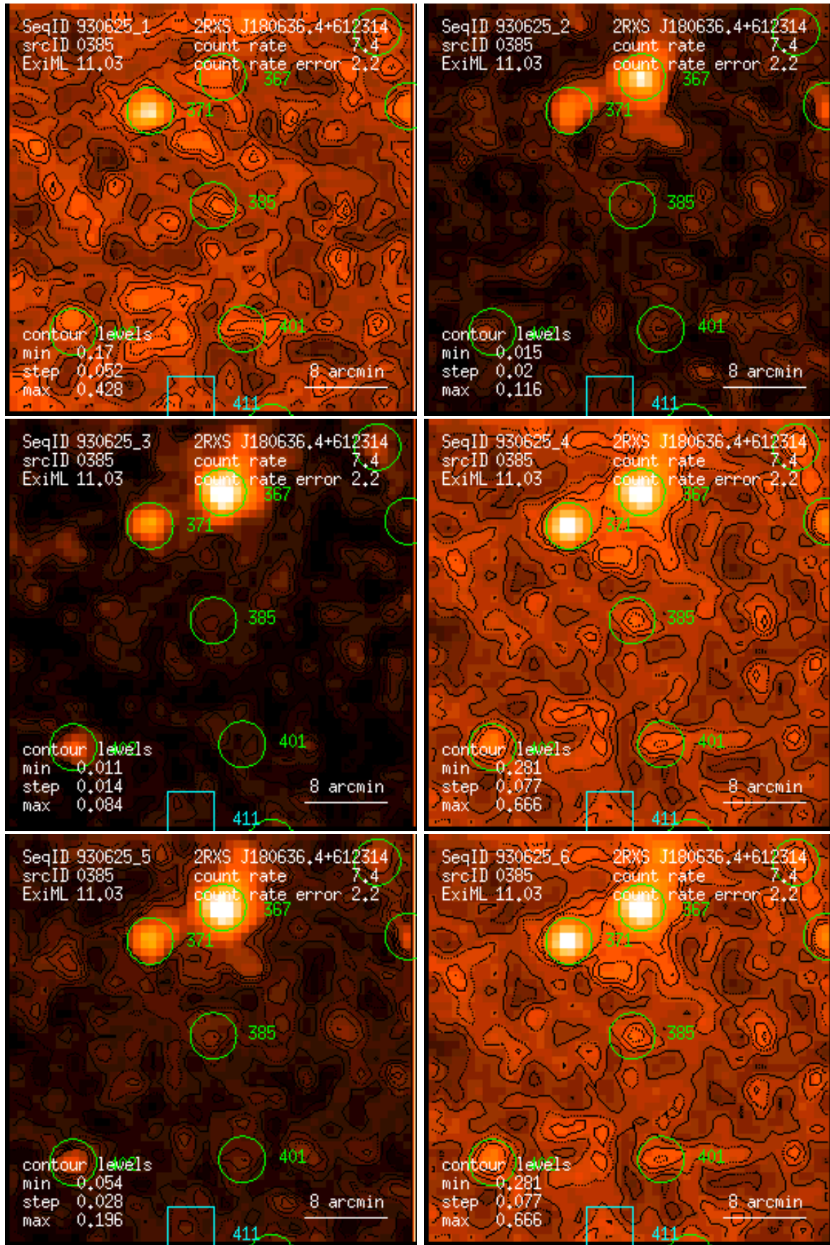
Figure 385: RASS 930625: detection 0385: band rate images, Gaussian filter: (1) PSPC channels 11 – 41, (2) 52 – 90, (3) 91 – 201, (4) 11 – 235, (5) 52 – 201, (6) 11 – 201. Broad band rates in counts/ks. Band rate contour levels in counts/ks/arcmin 2 .
