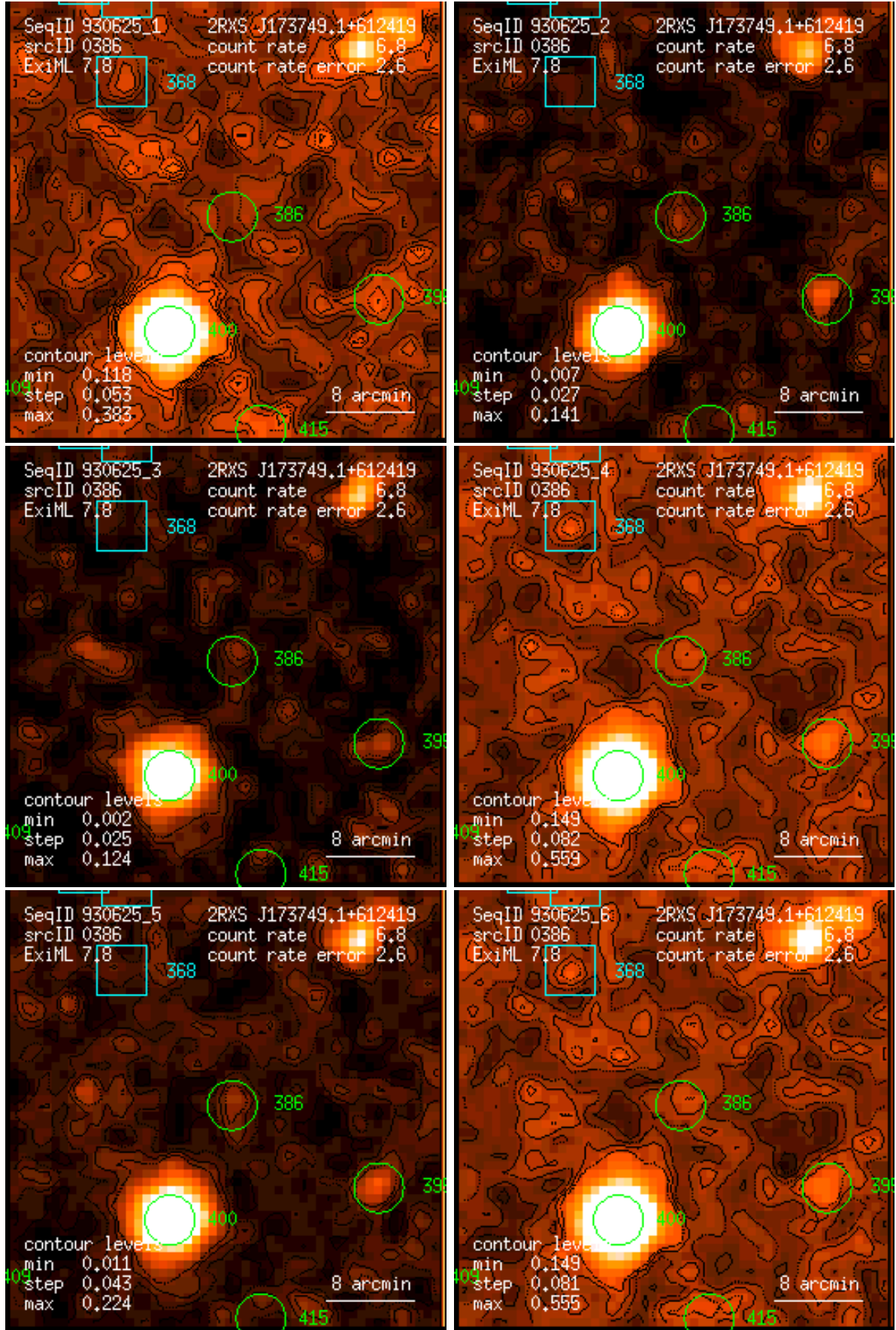
Figure 386: RASS 930625: detection 0386: band rate images, Gaussian filter: (1) PSPC channels 11 – 41, (2) 52 – 90, (3) 91 – 201, (4) 11 – 235, (5) 52 – 201, (6) 11 – 201. Broad band rates in counts/ks. Band rate contour levels in counts/ks/arcmin 2 .
