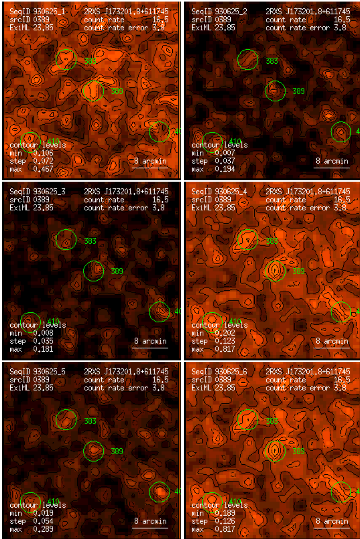
Figure 389: RASS 930625: detection 0389: band rate images, Gaussian filter: (1) PSPC channels 11 – 41, (2) 52 – 90, (3) 91 – 201, (4) 11 – 235, (5) 52 – 201, (6) 11 – 201. Broad band rates in counts/ks. Band rate contour levels in counts/ks/arcmin 2 .
