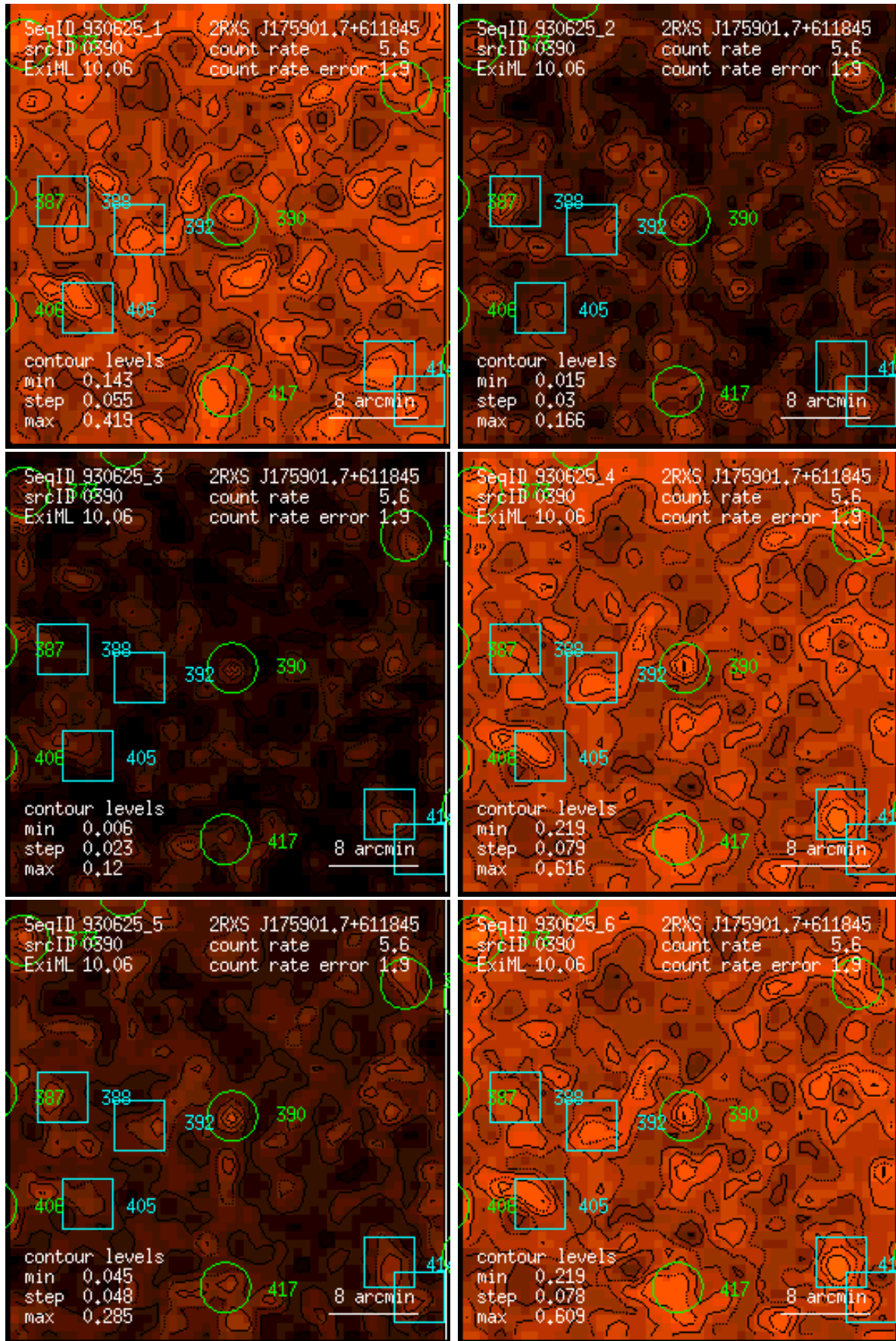
Figure 390: RASS 930625: detection 0390: band rate images, Gaussian filter: (1) PSPC channels 11 – 41, (2) 52 – 90, (3) 91 – 201, (4) 11 – 235, (5) 52 – 201, (6) 11 – 201. Broad band rates in counts/ks. Band rate contour levels in counts/ks/arcmin 2 .
