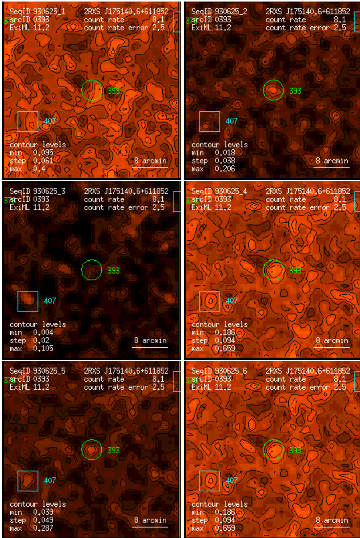
Figure 393: RASS 930625: detection 0393: band rate images, Gaussian filter: (1) PSPC channels 11 – 41, (2) 52 – 90, (3) 91 – 201, (4) 11 – 235, (5) 52 – 201, (6) 11 – 201. Broad band rates in counts/ks. Band rate contour levels in counts/ks/arcmin 2 .
