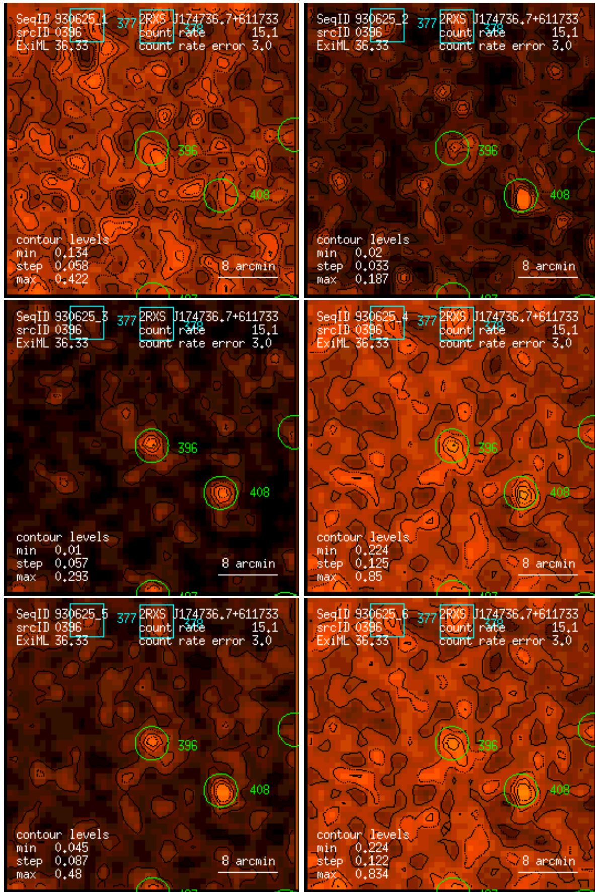
Figure 396: RASS 930625: detection 0396: band rate images, Gaussian filter: (1) PSPC channels 11 – 41, (2) 52 – 90, (3) 91 – 201, (4) 11 – 235, (5) 52 – 201, (6) 11 – 201. Broad band rates in counts/ks. Band rate contour levels in counts/ks/arcmin 2 .
