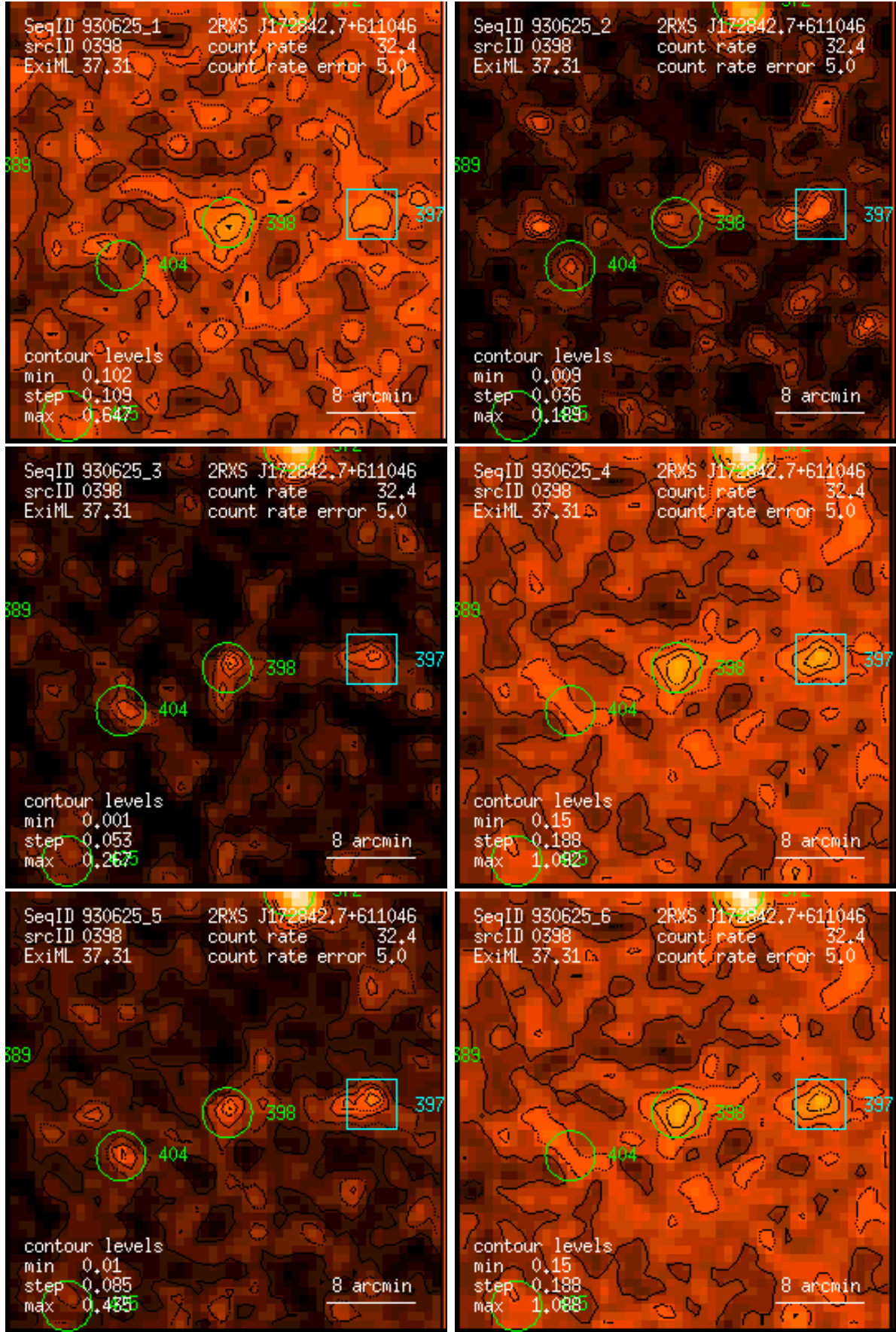
Figure 398: RASS 930625: detection 0398: band rate images, Gaussian filter: (1) PSPC channels 11 – 41, (2) 52 – 90, (3) 91 – 201, (4) 11 – 235, (5) 52 – 201, (6) 11 – 201. Broad band rates in counts/ks. Band rate contour levels in counts/ks/arcmin 2 .
